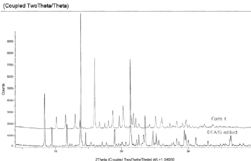
Fig. 4 XRPD of Form A polymorph and Form B polymorph of DEA solvate of Compound 1
