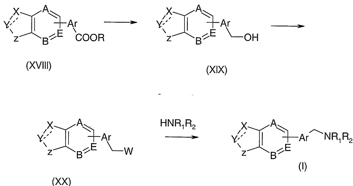
Scheme 8
