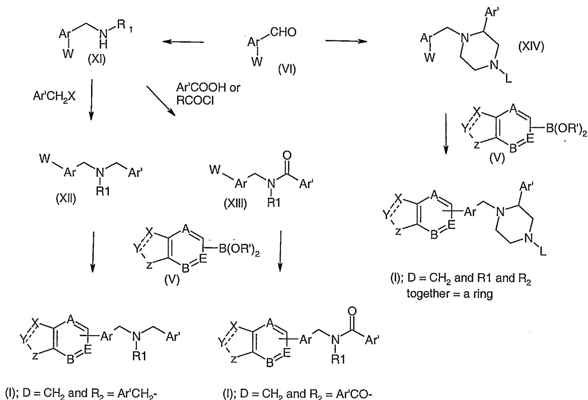
Scheme 5
