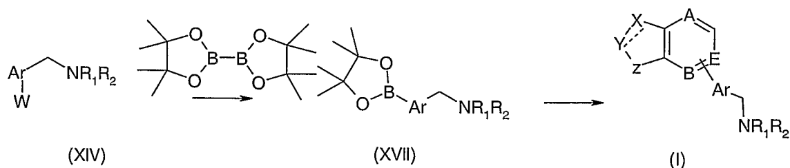
Scheme 7
