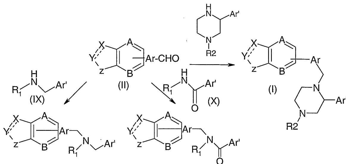
Scheme 4
