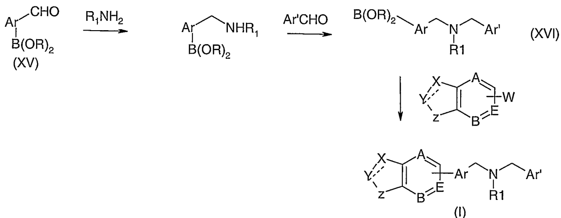
Scheme 6
