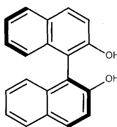
(S)-BINOL
