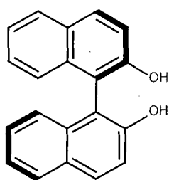
(R)-BINOL
