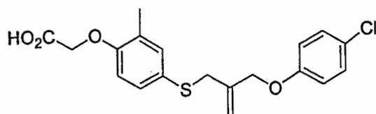
Compound 5
