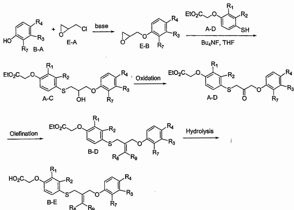
Scheme E
