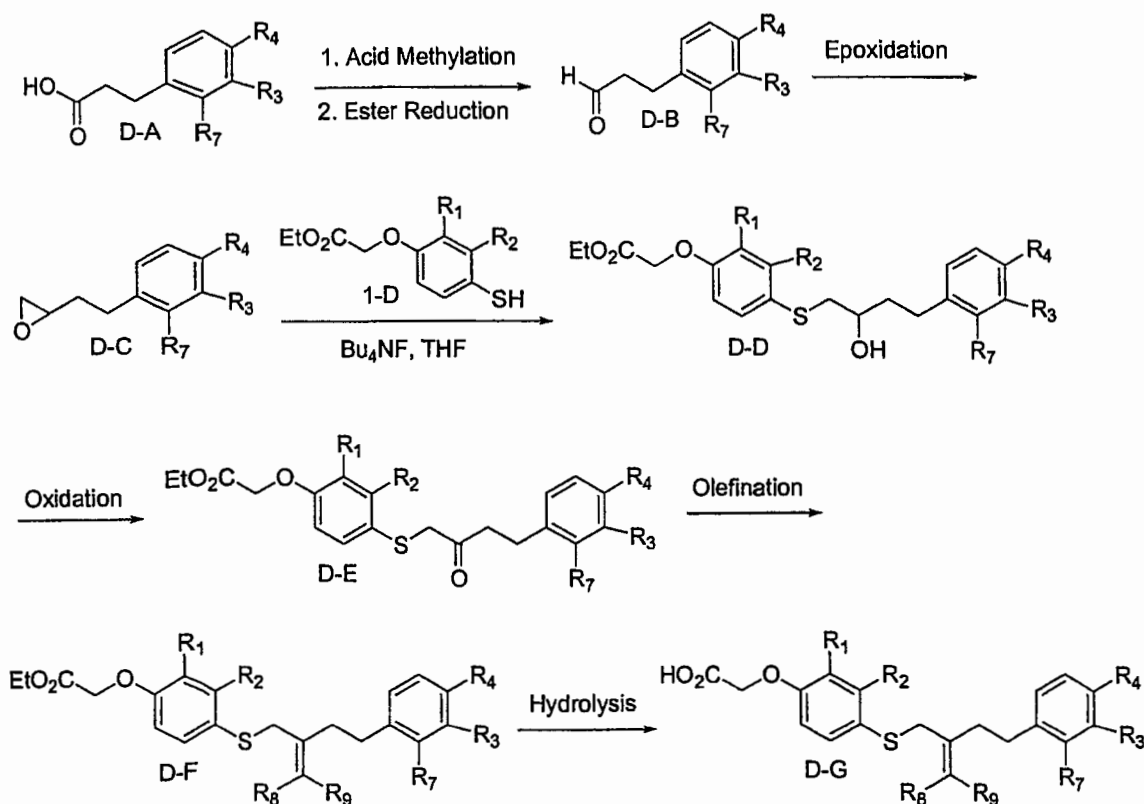
Scheme D
