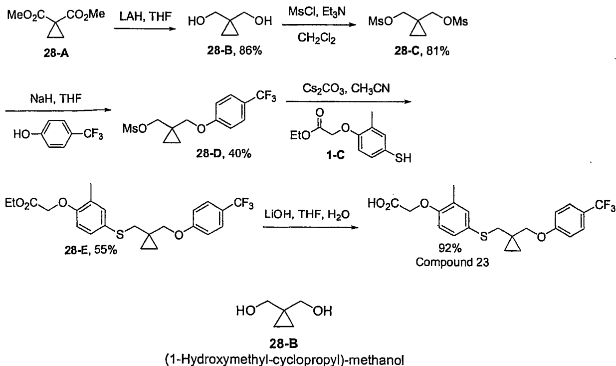
Scheme 28
