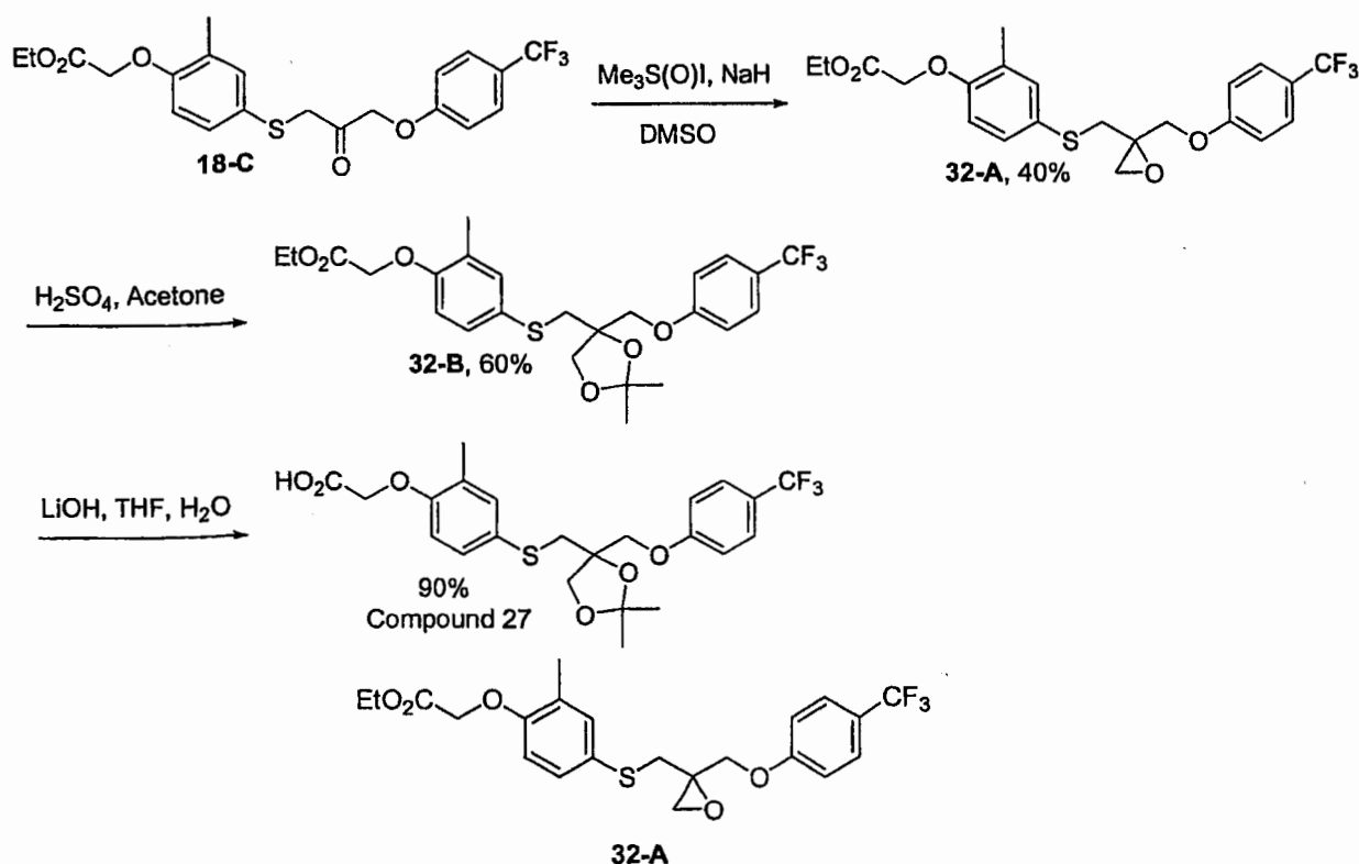
Scheme 32
