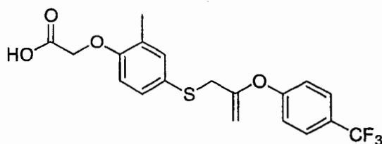
Compound 21
