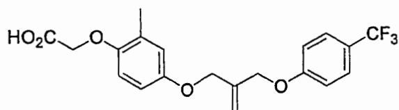
Compound 29
