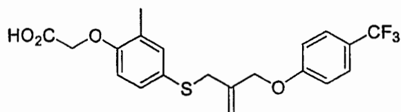
Compound 1
