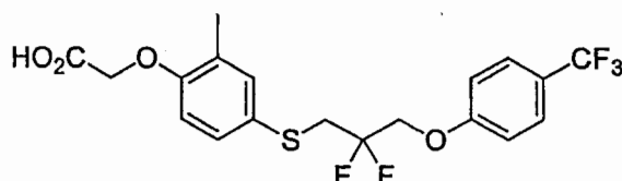
Compound 25
