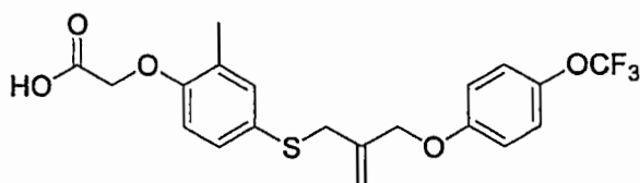
Compound 4
