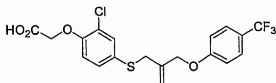
Compound 11
