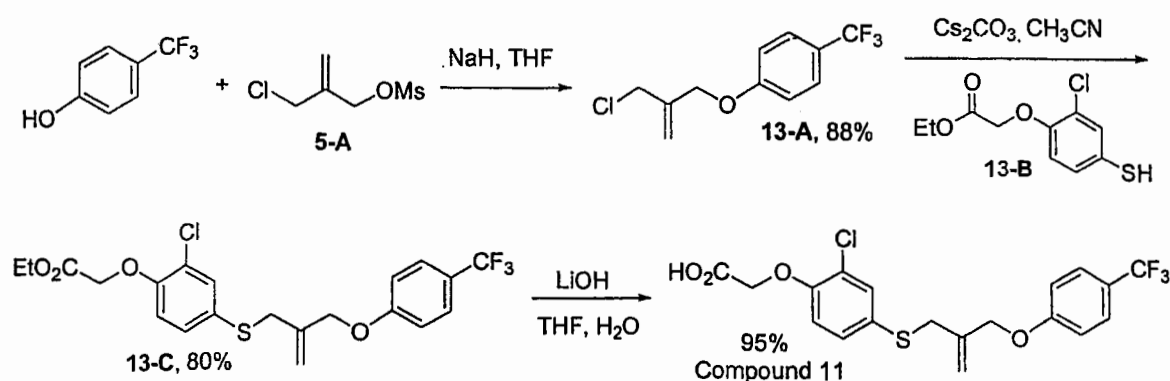
Scheme 13
