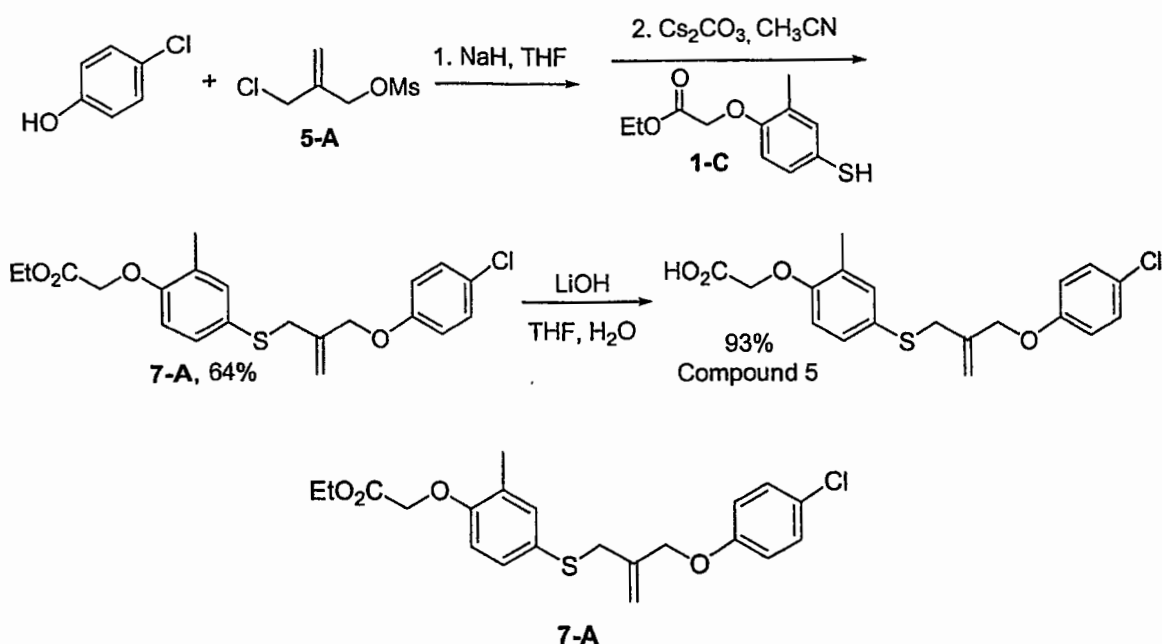
Scheme 7
