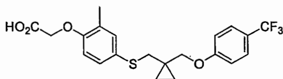
Compound 23
