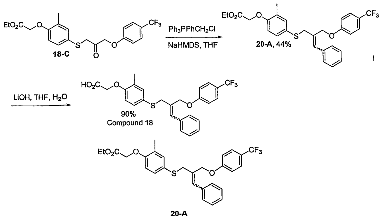
Scheme 20
