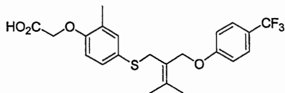
Compound 15
