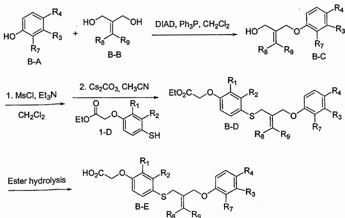
Scheme B
