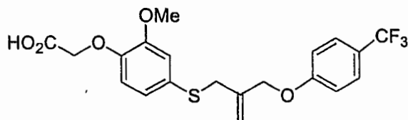
Compound 14
