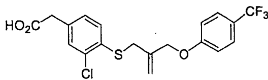
Compound 22
