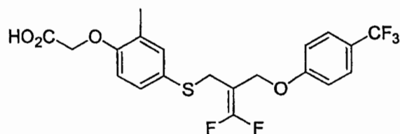
Compound 16
