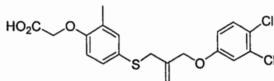
Compound 6
