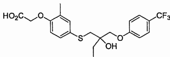
Compound 28
