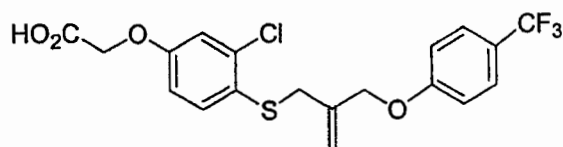
Compound 13
