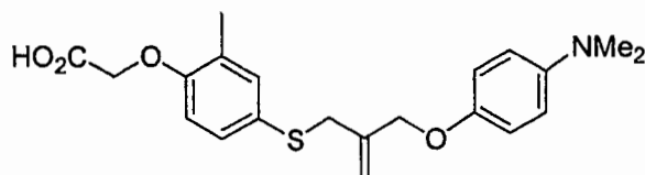
Compound 10
