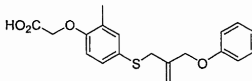
Compound 3
