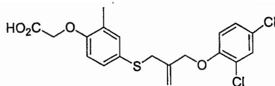
Compound 7
