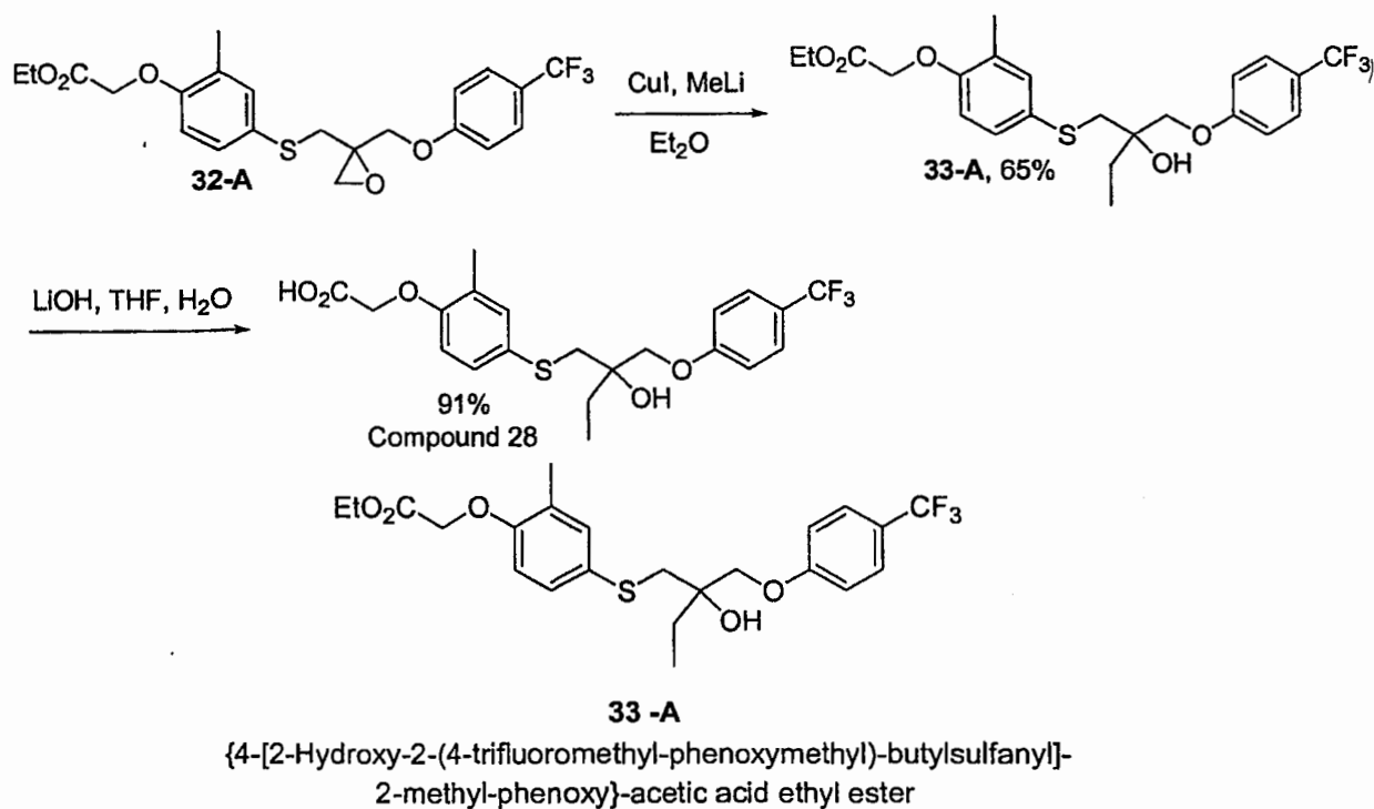
Scheme 33
