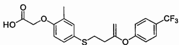
Compound 20
