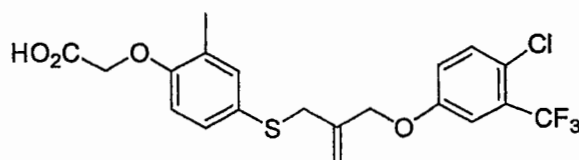
Compound 8
