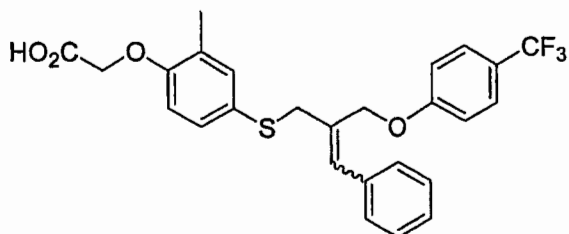
Compound 18
