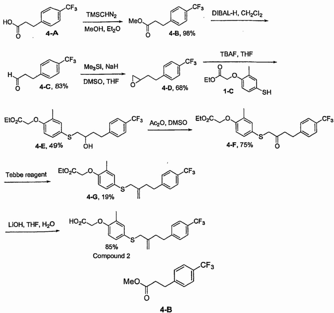
Scheme 4
