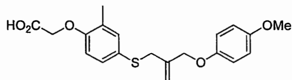
Compound 9
