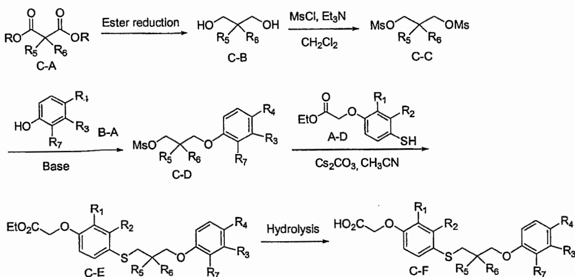
Scheme C
