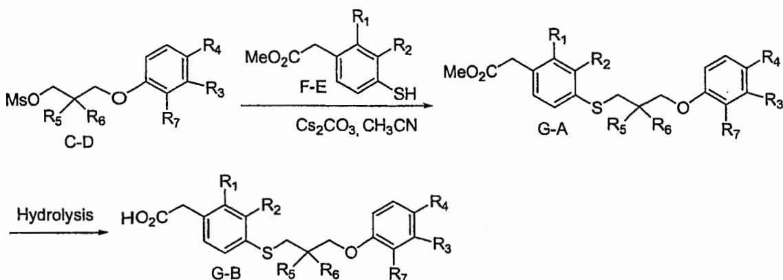
Scheme G
