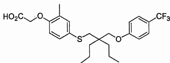
Compound 24
