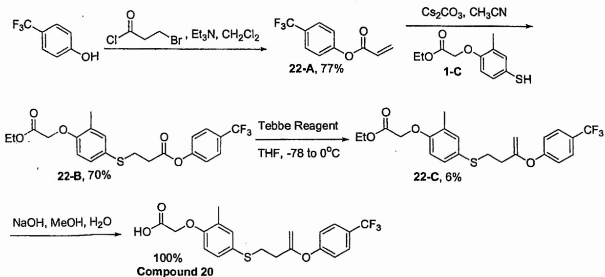
Scheme 22
