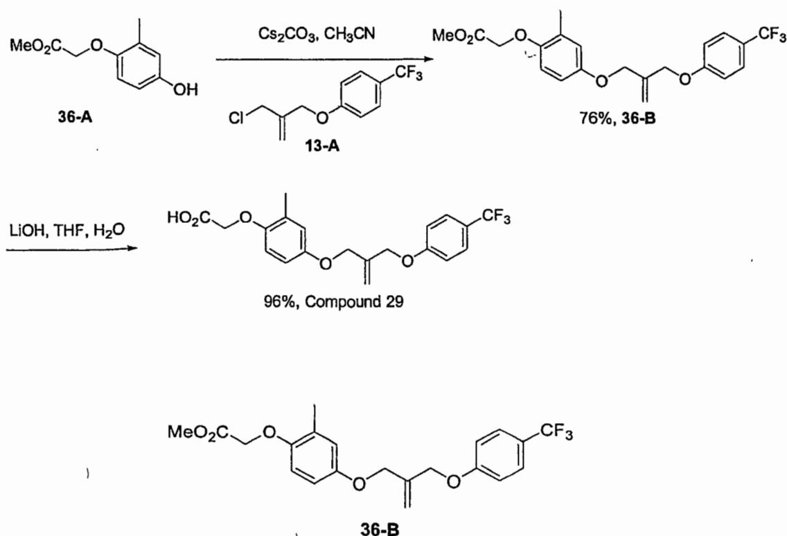
Scheme 36
