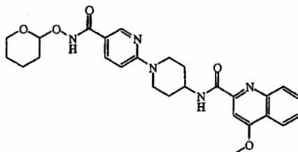
intermediate 3
