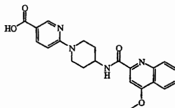
intermediate 2
