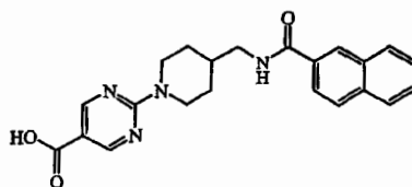
.Na intermediate 7
