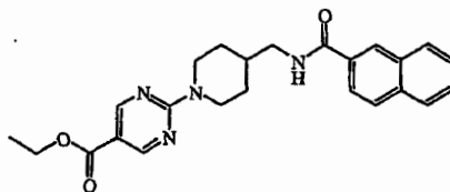
intermediate 6
