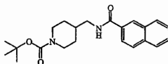
intermediate 4
