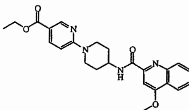
intermediate 1
