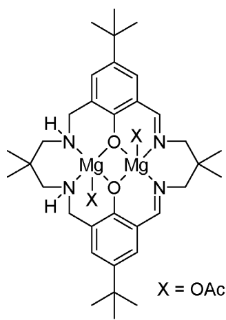
[L^{imine^8}Mg_2(OAc_2)]
