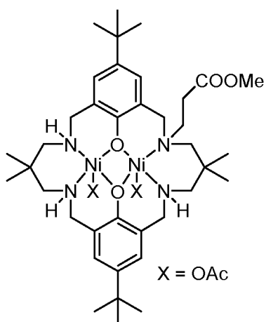
L^{12}Ni_2(OAc)_2
