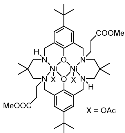
L^{13}Ni_2(OAc)_2
