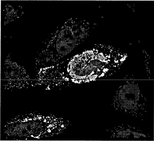
ScFv-PD-L1-TOM7
