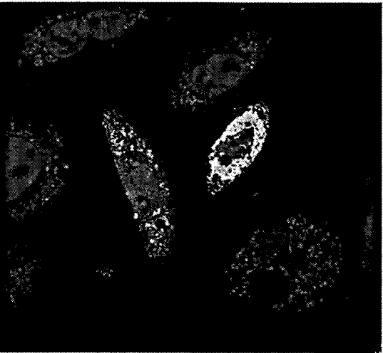
ScFv-HER2-TOM7
