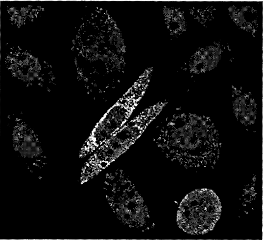
ScFv-MEL-TOM7
