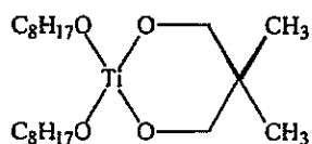
Di(2-ethyl-1-hexyl) 2,2-dimethylpropane-1,3-dioxytitanate
