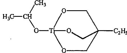
1-(2-Propoxy)-4-ethyl-2,6,7-trioxabicyclo[2,2,2]octane
