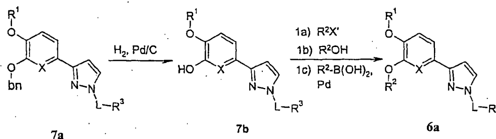
Scheme 3
