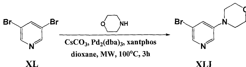
Scheme 7
