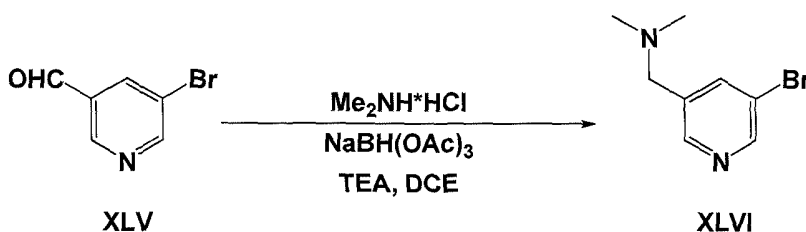
Scheme 10
