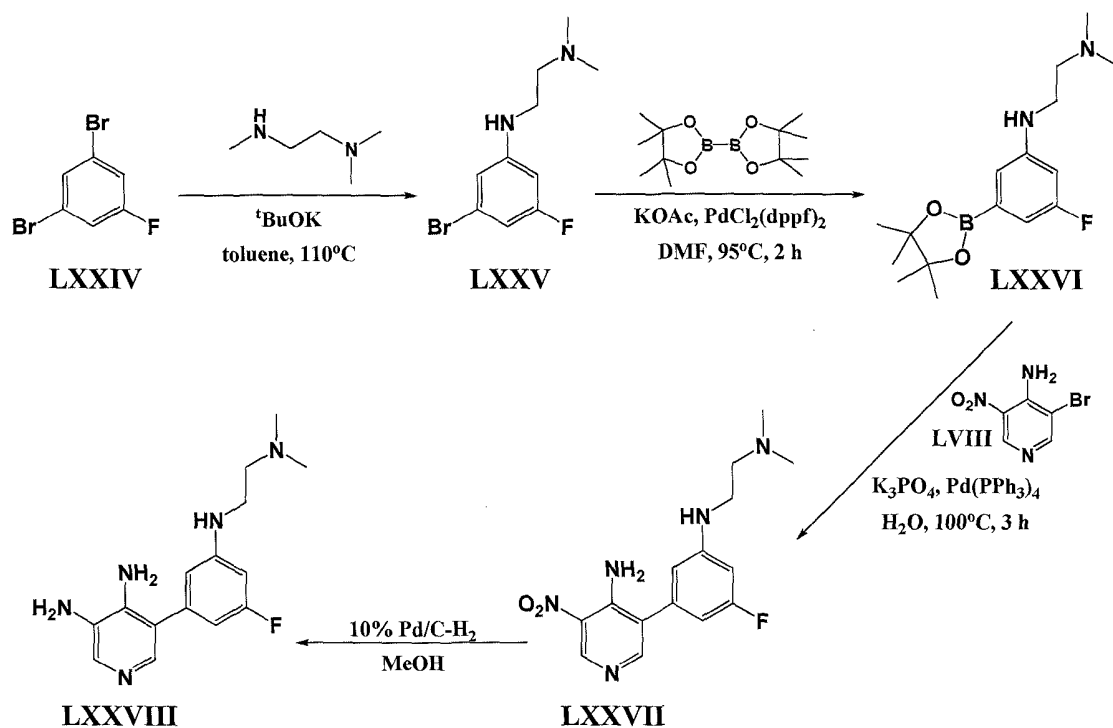
Scheme 14
