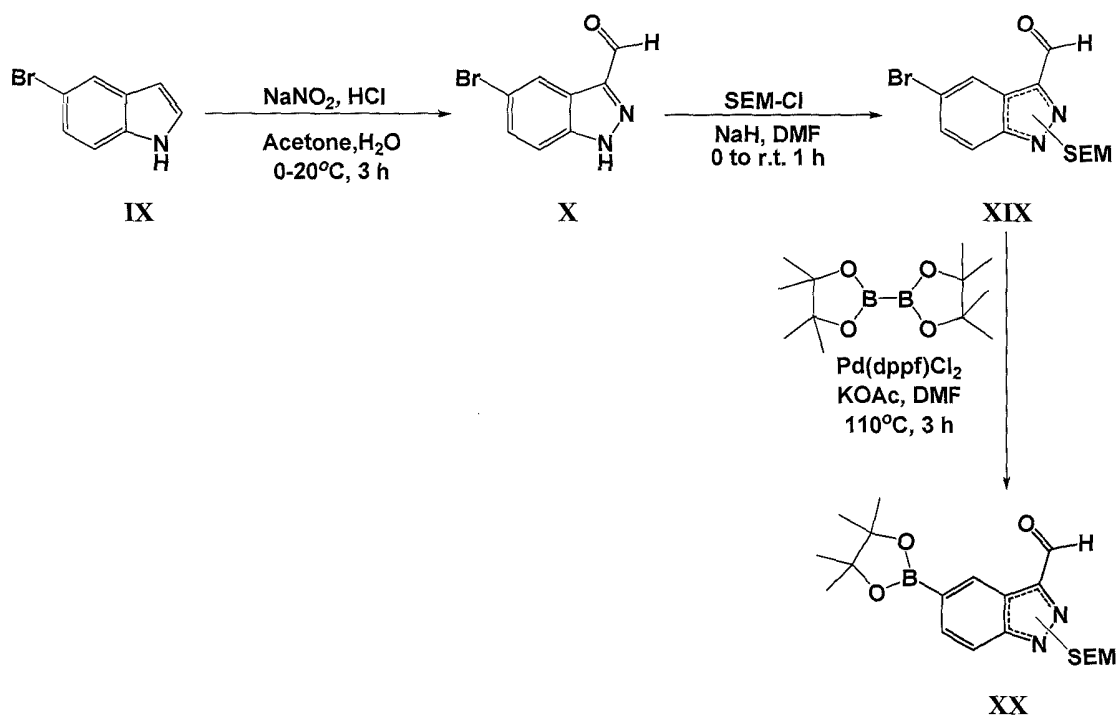
Scheme 4
