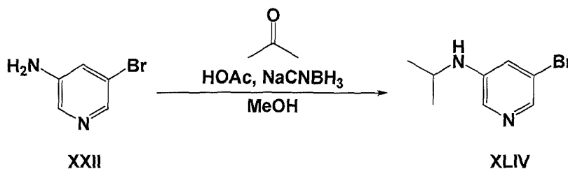
Scheme 9
