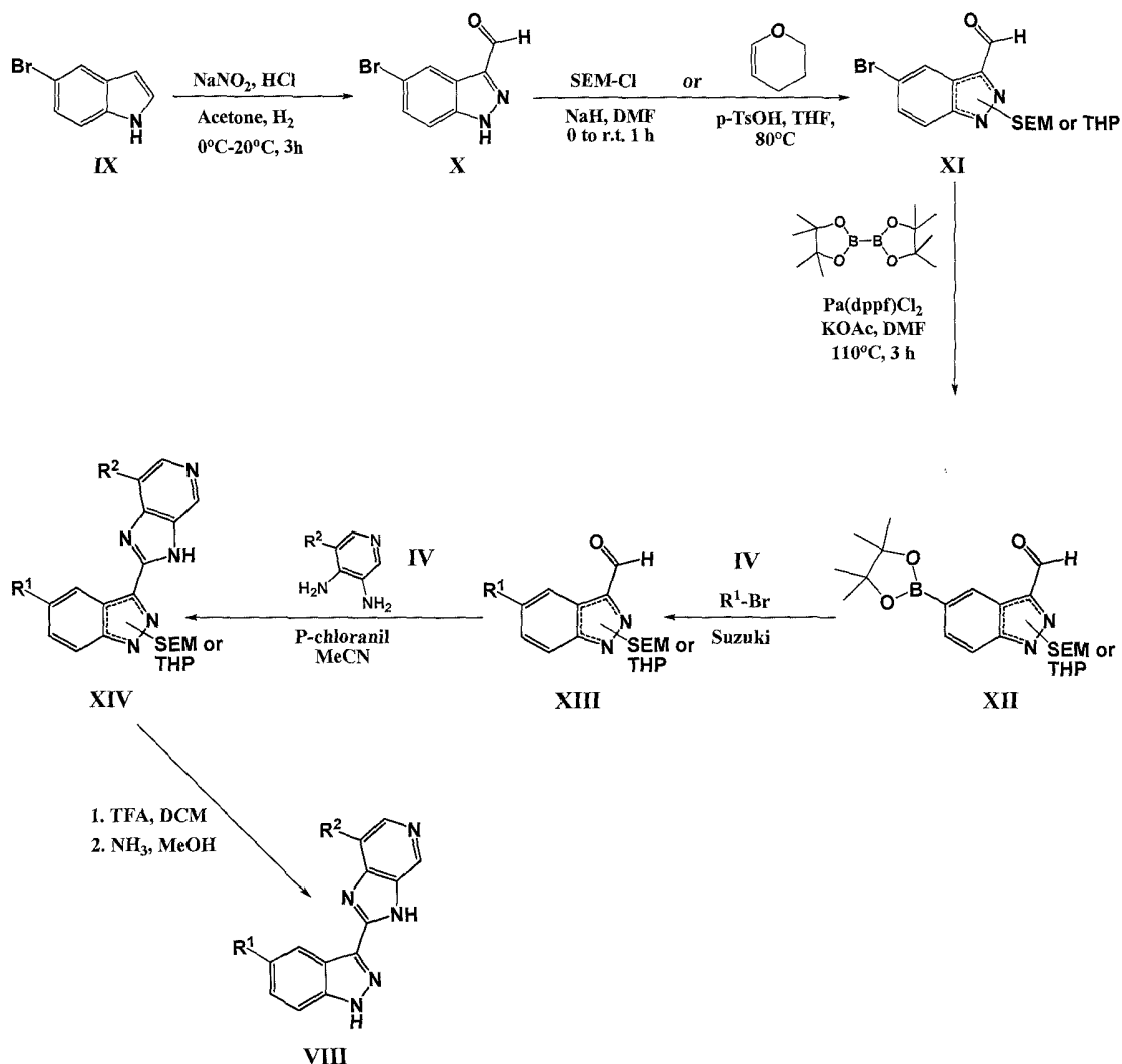
Scheme 2
