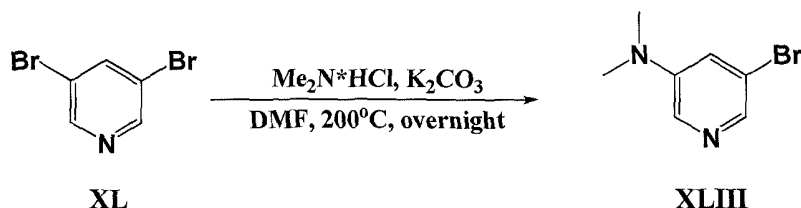
Scheme 8
