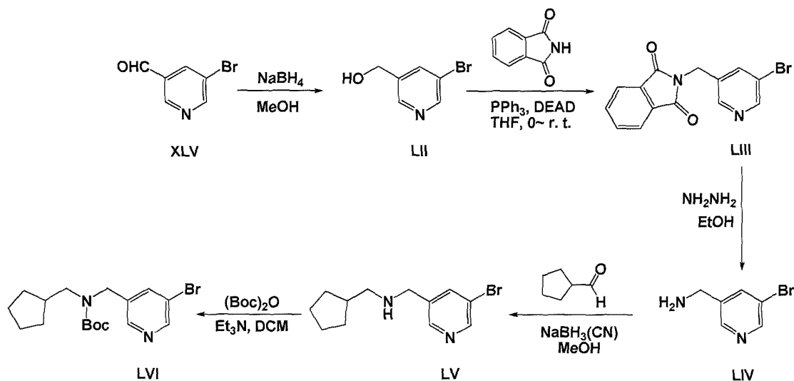
Scheme 11
