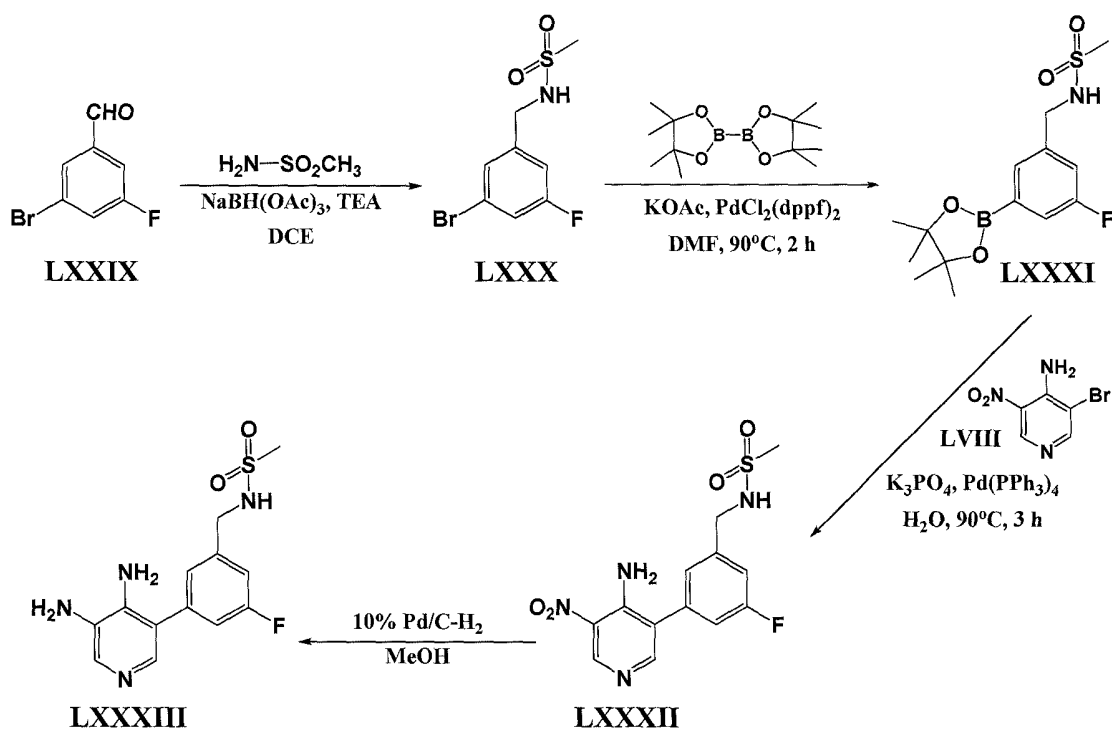
Scheme 15
