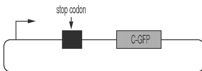
Fluorescent reporter
