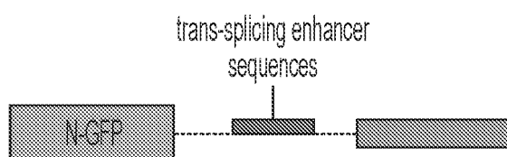
Trans-splicing RNA
