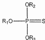
Formula B
