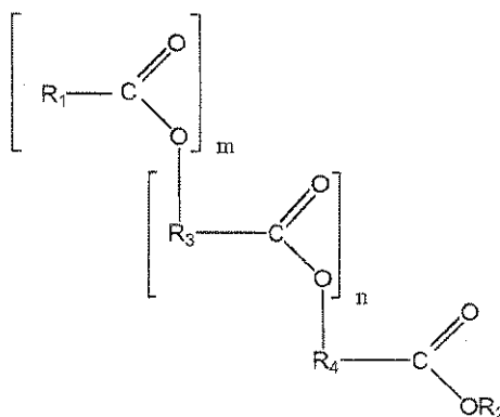
Formula II
