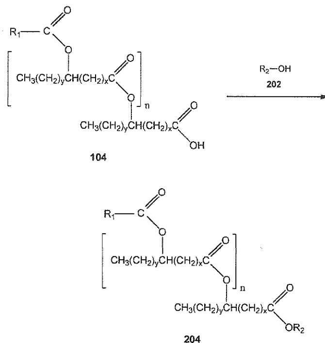
Scheme 2
