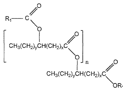
Formula III
