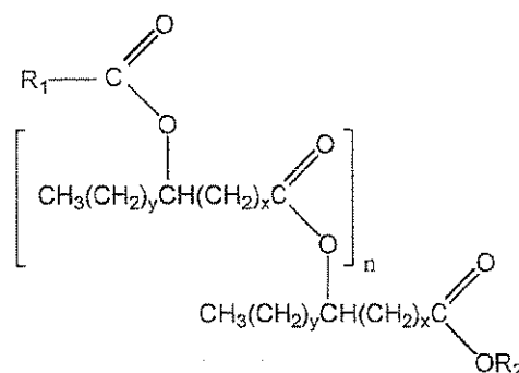
Formula III
