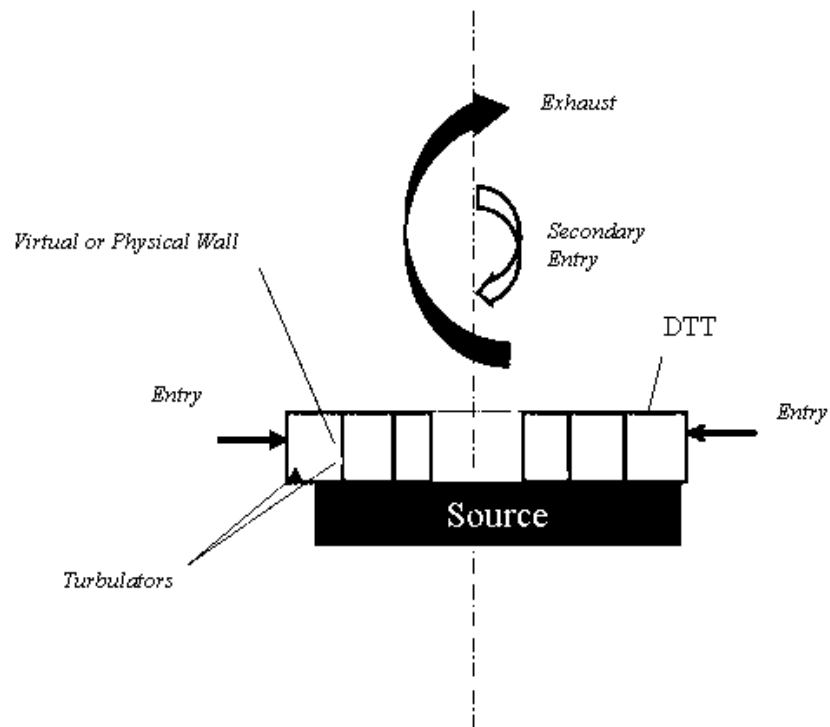
Fig 3 Sectional View, with examples of geometry and locations of turbulators
