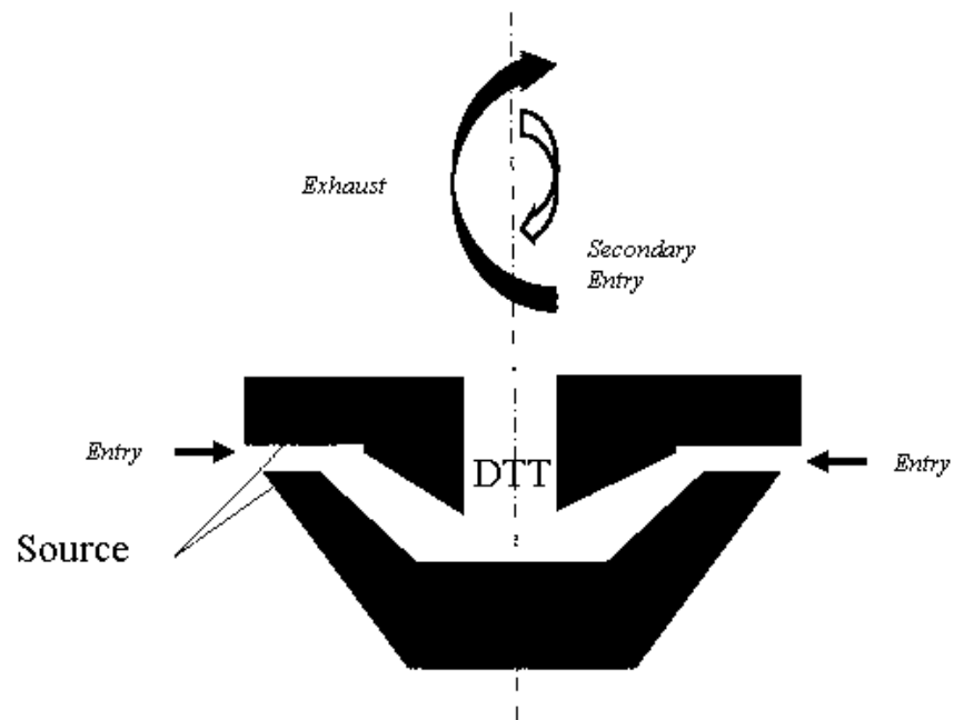
Fig 7 Non-planner Source, Encapsulated within Source, variation 2
