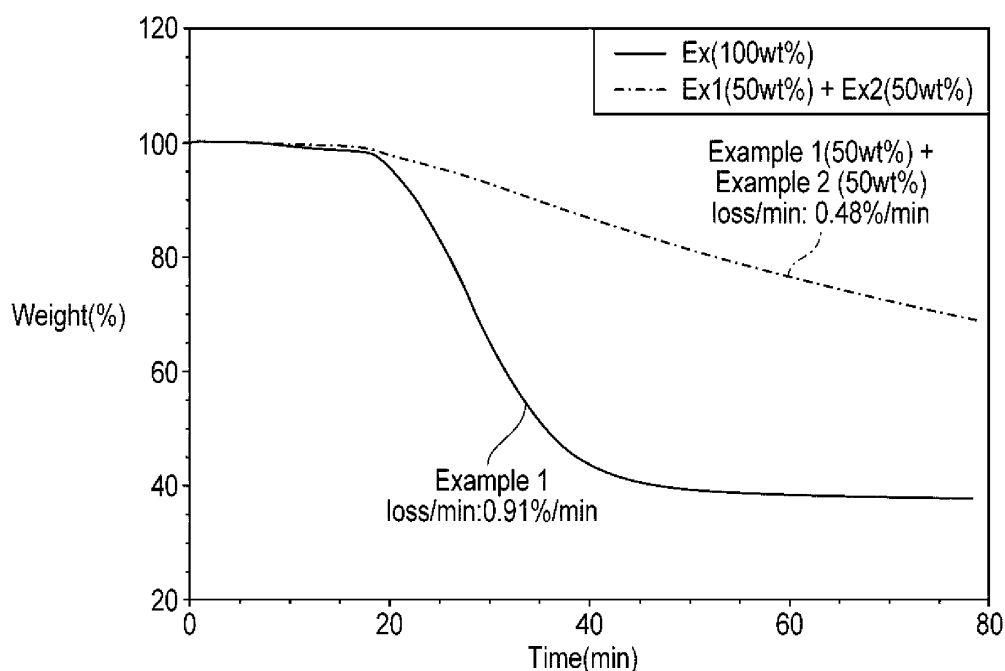
FIG. 3: Comparison of the isothermal baking behavior of Example 1 vs. a mixture of Example 1 (50wt%) and Example 2 (50wt%).
