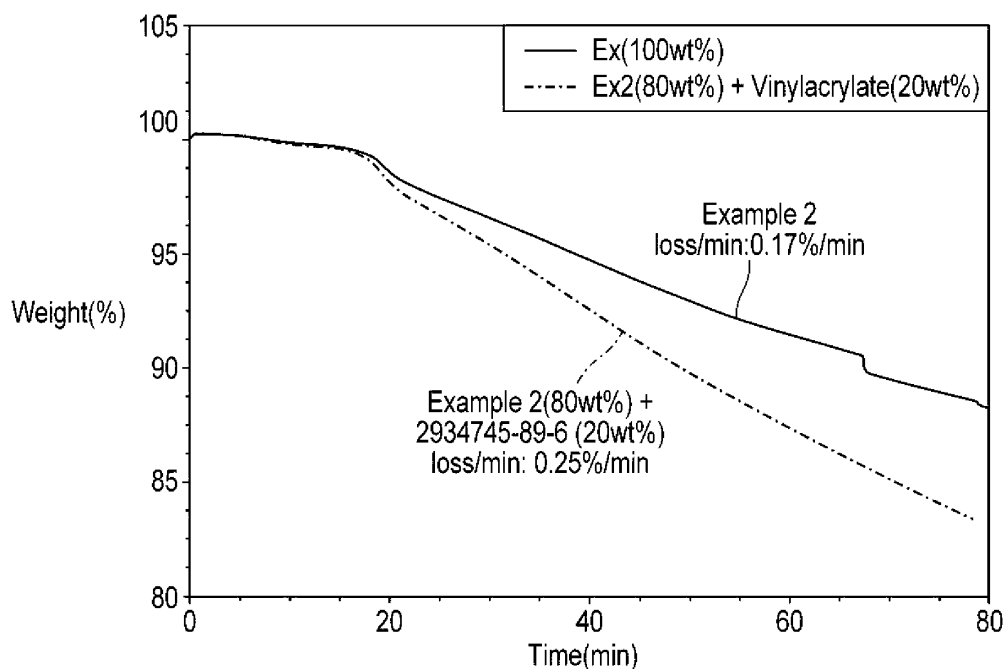
FIG. 4: Comparison of the isothermal baking behavior of Example 2 vs. a mixture of Example 2 (80wt%) and CAS: 2934745-89-6 (20wt%).
