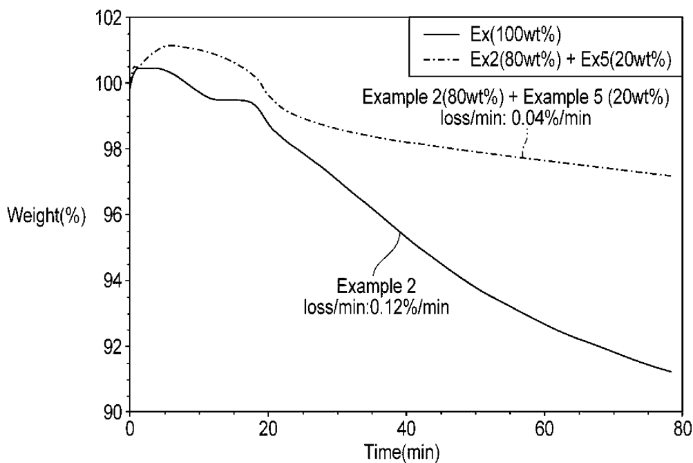
FIG. 2: Comparison of the isothermal baking behavior of Example 2 vs. a mixture of Example 2 (80wt%) and Example 5 (20wt%).
