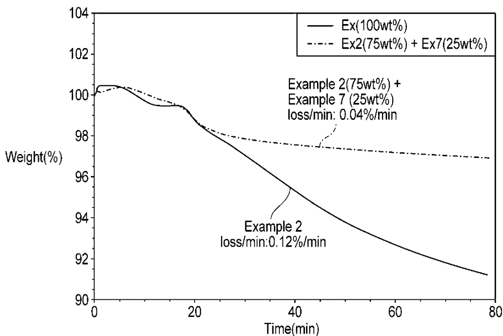
FIG. 1: Comparison of the isothermal baking behavior of Example 2 vs. a mixture of Example 2 (75wt%) and Example 7 (25wt%).
