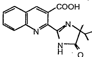
imazaquin
