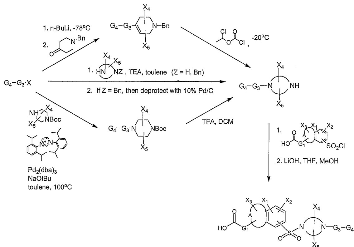
Scheme IX
