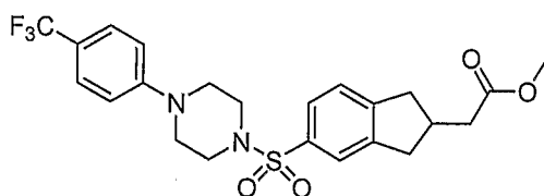
{5-[4-(4-Trifluoromethyl-phenyl)-piperazine-1-sulfonyl]-indan-2-yl}-acetic acid methyl ester:
