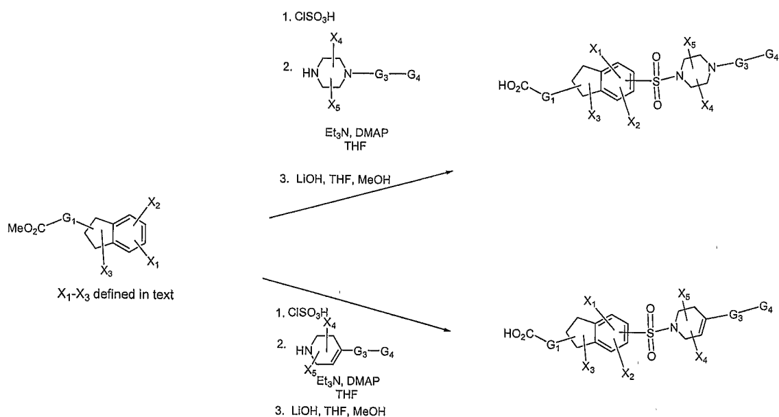
Scheme I
