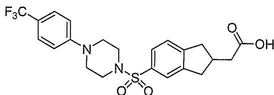
{5-[4-(4-Trifluoromethyl-phenyl)-piperazine-1-sulfonyl]-indan-2-yl}-acetic acid
