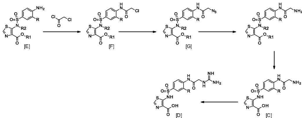
Scheme 3
