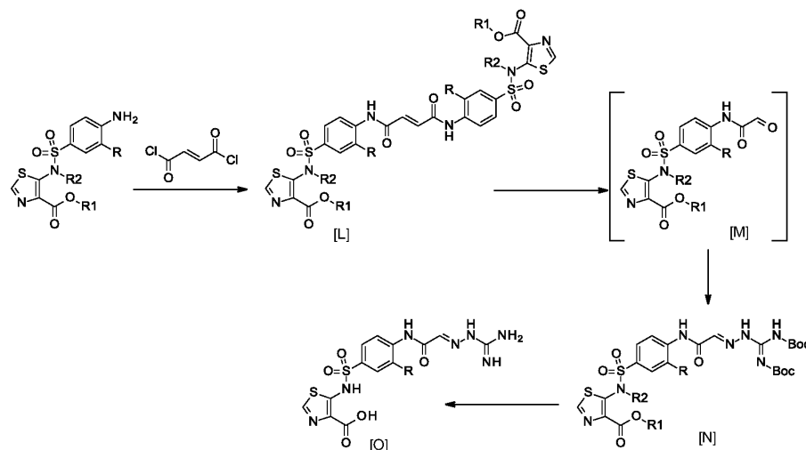
Scheme 5
