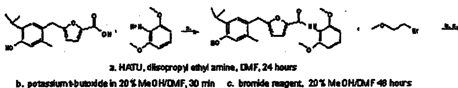
Compound B
