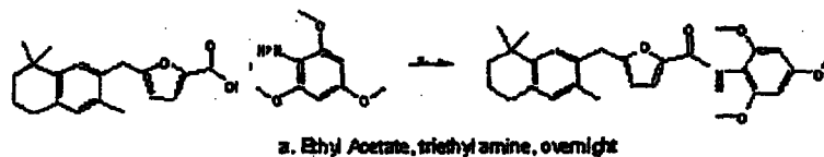
Compound A
