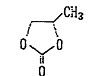
propylene carbonate (PC)
