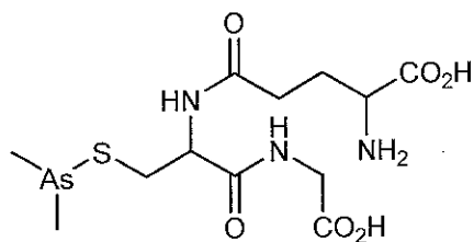
Compound A
