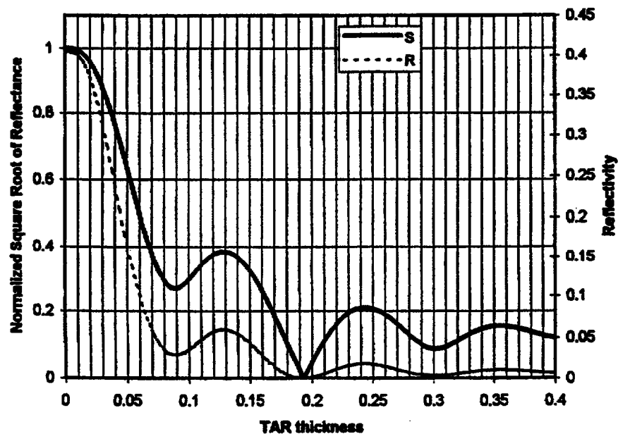
Figure 4: Swing ratio and reflectivity for n = 1.65 and k = 0.30 . Silicon substrate, photoresist refractive index N_r = 1.704 - 0.024 .
