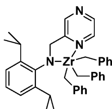
Procatalyst 2
