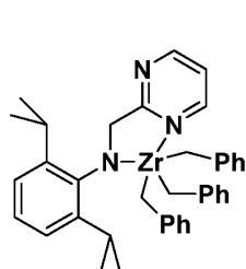
Procatalyst 1
