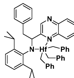
Procatalyst 6
