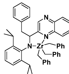
Procatalyst 3
