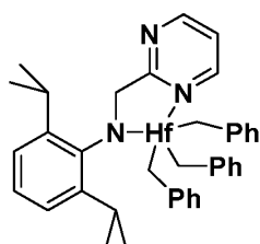
Procatalyst 4
