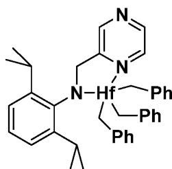
Procatalyst 5
