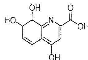
7,8-dihydro-7,8-dihydroxykynurenic acid
