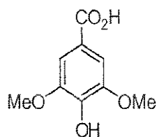
syringic acid
