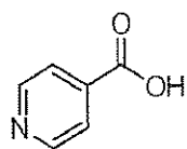
isonicotinic acid
