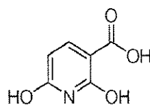
2,6-dihydroxynicotinic acid
