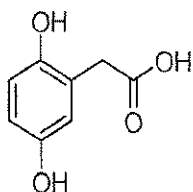
homogentisic acid
