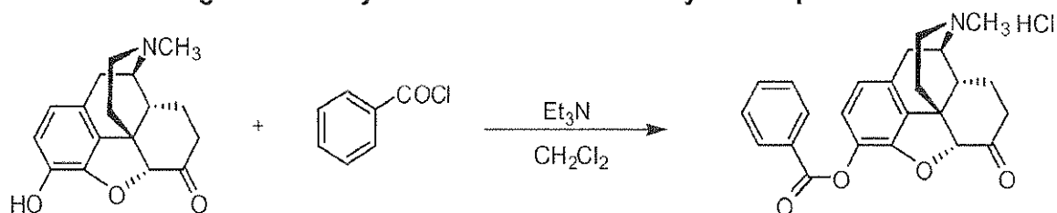
Figure 21C: Synthesis of 3-benzoate-hydromorphone:
