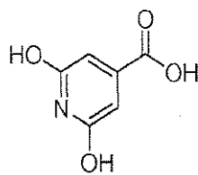
citrazinic acid
