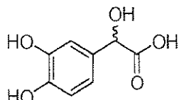
3,4-dihydroxymandelic acid
