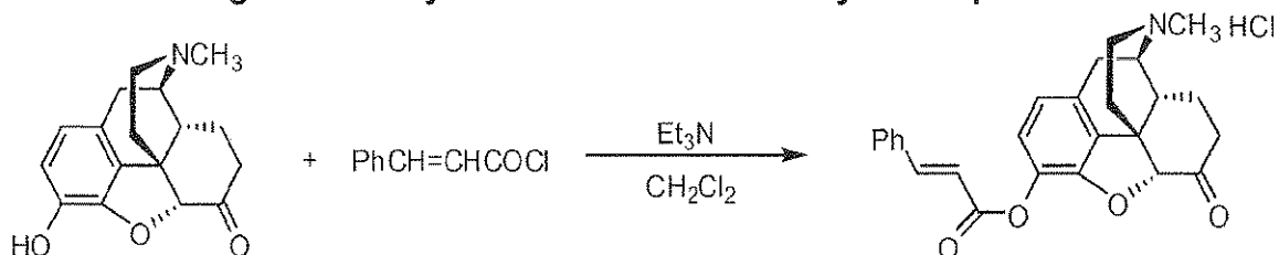
Figure 21B: Synthesis of 3-cinnamate-hydromorphone:
