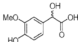
vanillylmandelic acid
