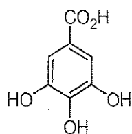
gallic acid
