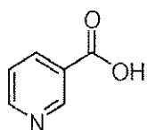
nicotinic acid
