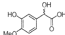
isovanillylmandelic acid
