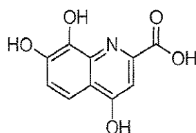
7,8-dihydroxykynurenic acid
