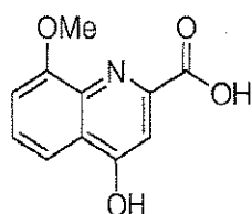
8-methoxykynurenic acid
