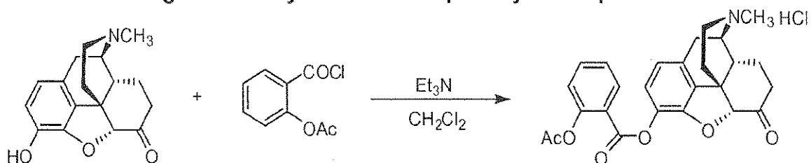
Figure 21A: Synthesis of 3-aspirin-hydromorphone:
