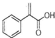
atropic acid
