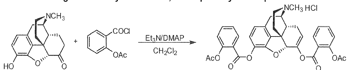
Figure 21D: Synthesis of 3,6-di-aspirin-hydromorphone:
