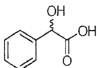
mandelic acid
