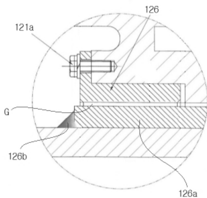
Detail of "A" Scale 5 : 1
