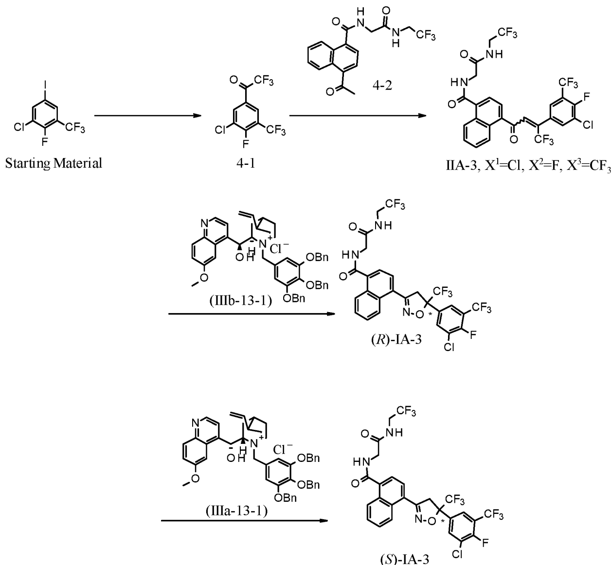
Scheme 4
