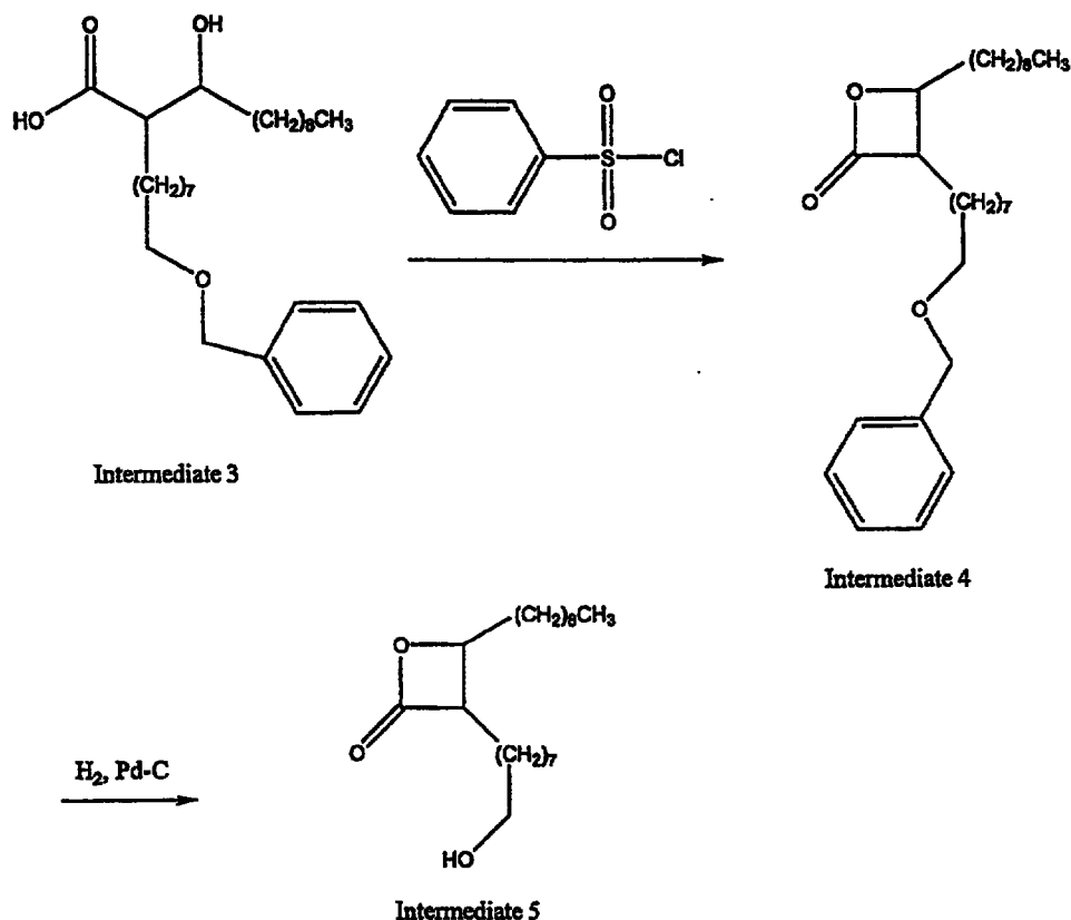
Scheme I: Synthesis of Intermediate 5.
