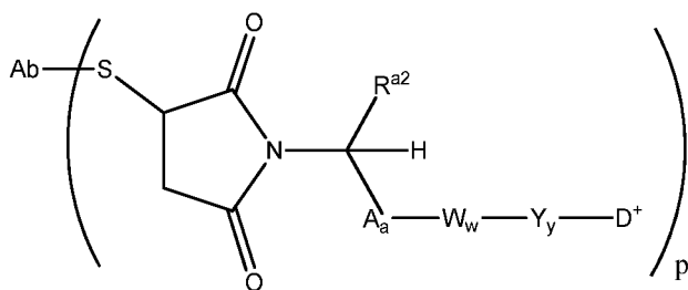
(Ab-S-Formula 1)
