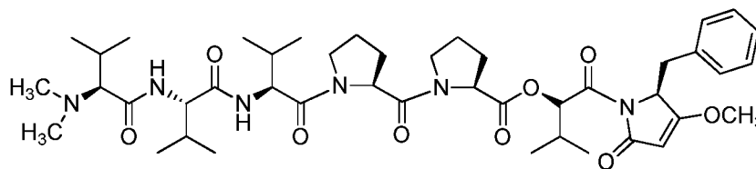
Dolastatin 15
