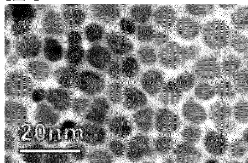
Co-Pt-Bi-TiO 2 -SiO 2
