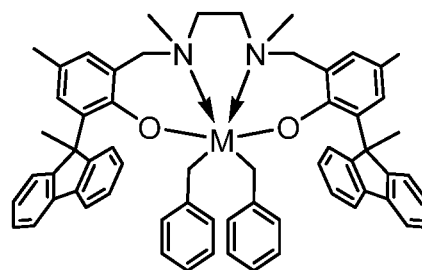
Structures of CAT-1, CAT-2, CAT-3 and CAT-4
