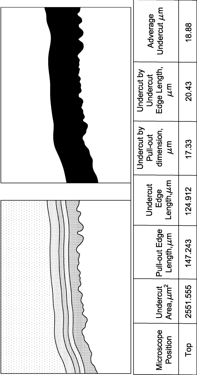
Standard Process (Center Only)
