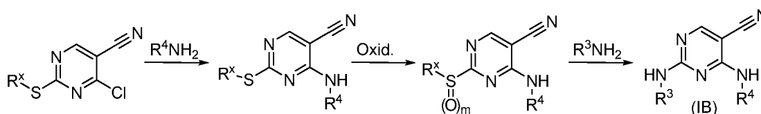
Scheme 9
