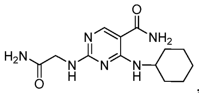
2-(2-aminoethylamino)-4-(cyclohexylamino)pyrimidine-5-carboxamide
