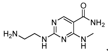
2-(2-aminopropylamino)-4-(cyclohexylamino)pyrimidine-5-carboxamide
