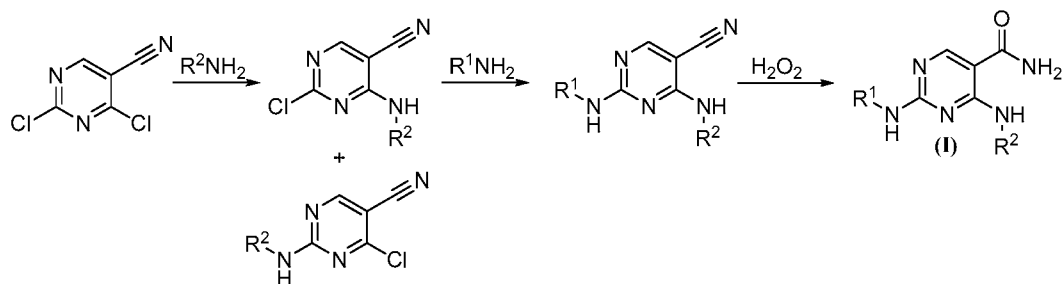
Scheme 4
