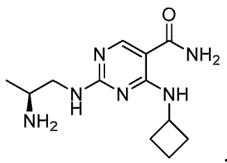
(S)-2-(2-aminopropylamino)-4-(cyclobutylamino)pyrimidine-5-carboxamide
