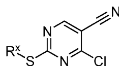
(VIIc),
