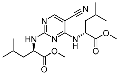
(2S,2'S)-diethyl 2,2'-(5-cyanopyrimidine-2,4-diyl)bis(azanediyl)-bis(3-methylbutanoate)
