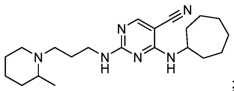
4-(4-methylcyclohexylamino)-2-(3-(2-methylpiperidin-1-yl)propylamino)-pyrimidine-5-carbonitrile
