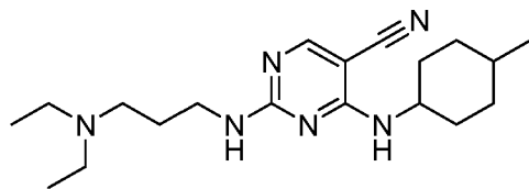
2-(3-(diethylamino)propylamino)-4-(4-methylcyclohexylamino)pyrimidine-5-carbonitrile
