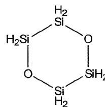
1,4-dioxo-2,3,5,6-tetrasilacyclohexane
