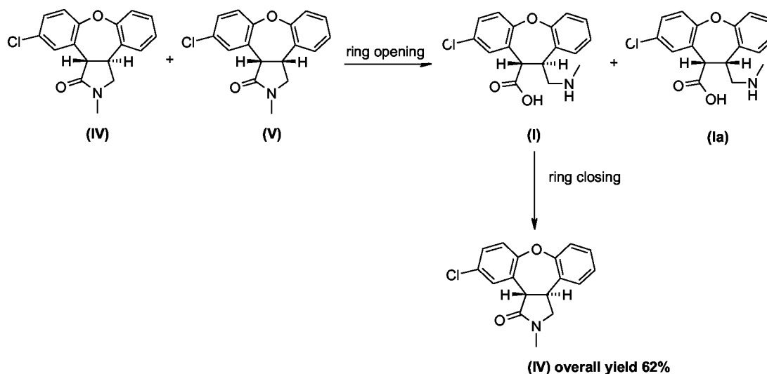
Scheme III
