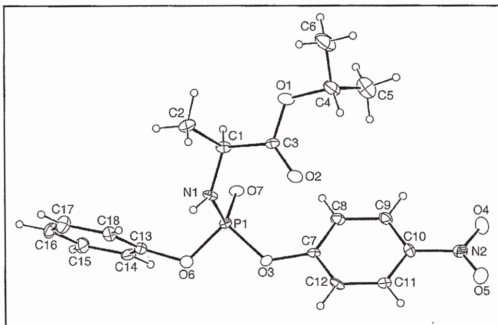
Figure 1A. ORTEP drawing of molecule no. 1 109 of the asymmetric unit with 30% probability thermal ellipsoids.
