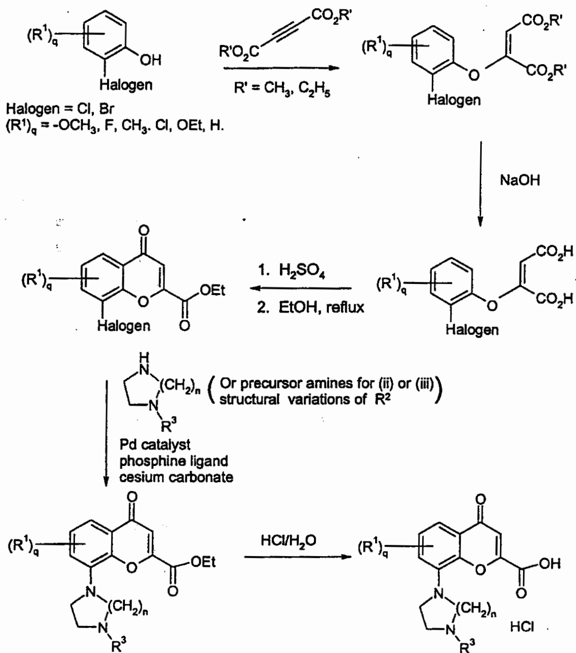
Scheme 1: Preparation of chromone-2-carboxylic acids as intermediates in the synthesis of compounds of the present invention.
