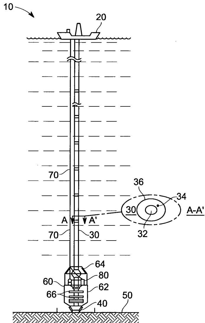
FIG. 1 (PRIOR ART)
