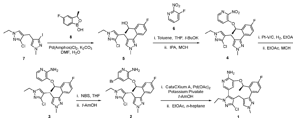
Scheme 4B. Synthesis of Compound 1.
