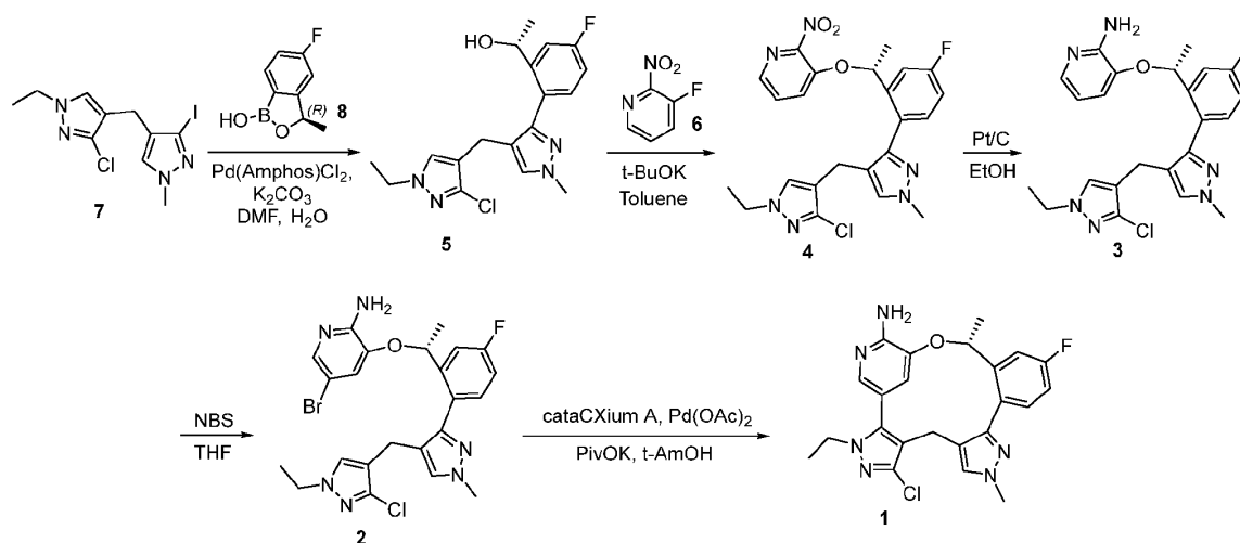
Scheme 4A. Synthesis of Compound 1.
