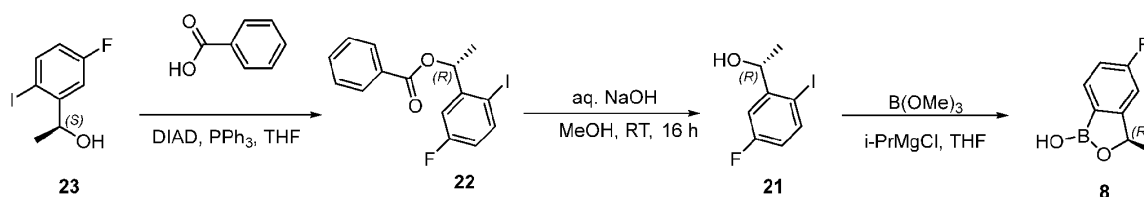
Scheme 1. Synthesis of Compound 8.
