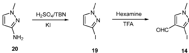
Scheme 7. Alternative Synthesis of Compound 14.
