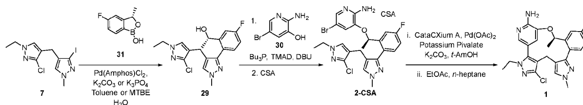
Scheme 9. Alternative Synthesis of Compound 1.
