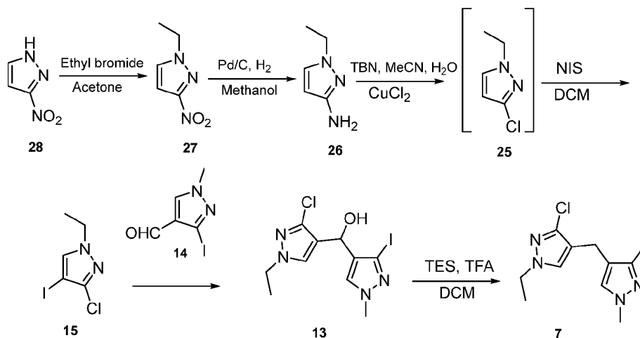
Scheme 8. Alternative Synthesis of Compound 7.
