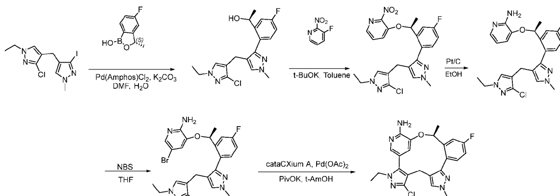
Scheme 5. Synthesis of Enantiomer of Compound 1.
