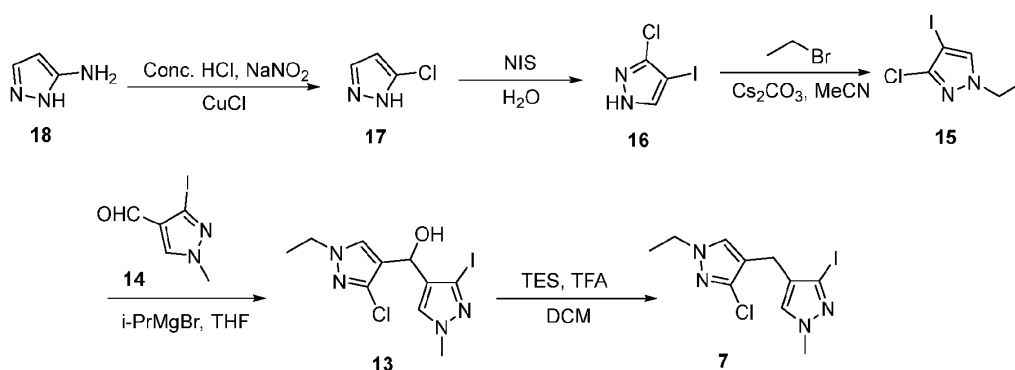
Scheme 3. Synthesis of Compound 7.
