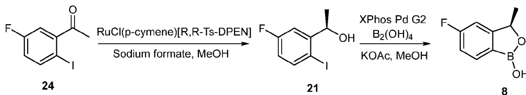
Scheme 6. Alternative Synthesis of Compound 8.
