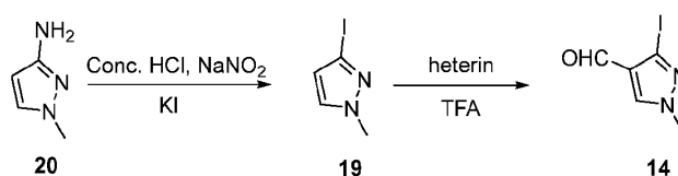
Scheme 2. Synthesis of Compound 14.
