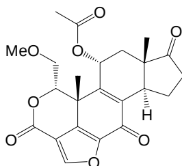
Wortmannin
