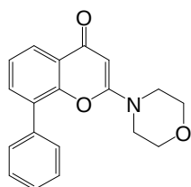
LY294002
