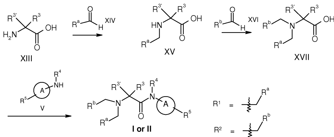
Scheme 4
