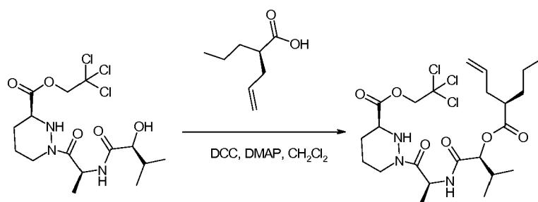
Compound 4d
