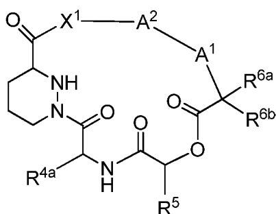
Formula II
