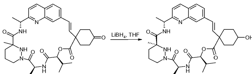
Compound 94.
