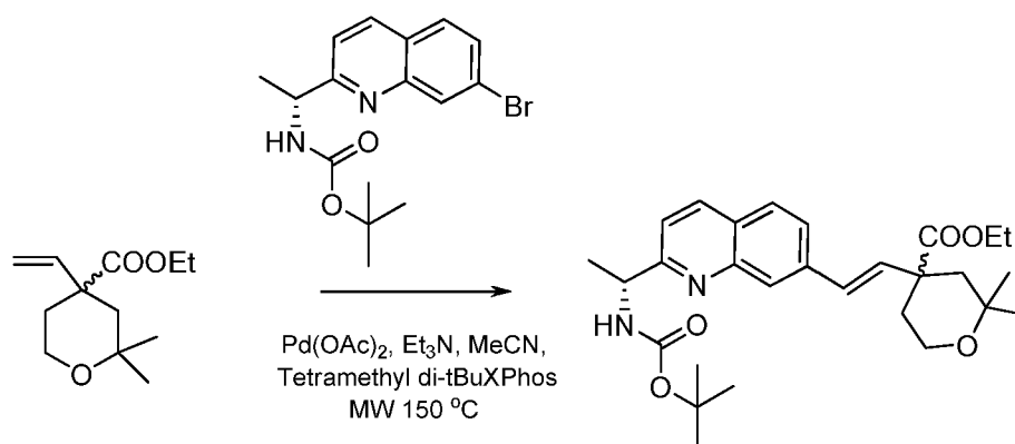
Compound 90a
