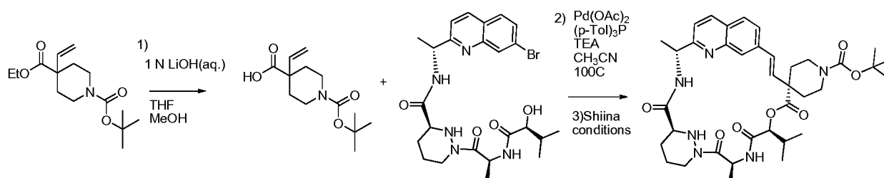
Compound 84
