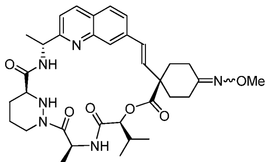
Compound 83a
