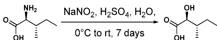
Compound 65a
