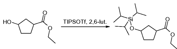
Compound 102a. 3-Triisopropylsilanyloxy-cyclopentanecarboxylic acid ethyl ester
