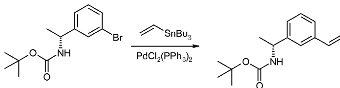
Compound 1i
