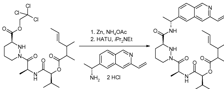
Compound 11d
