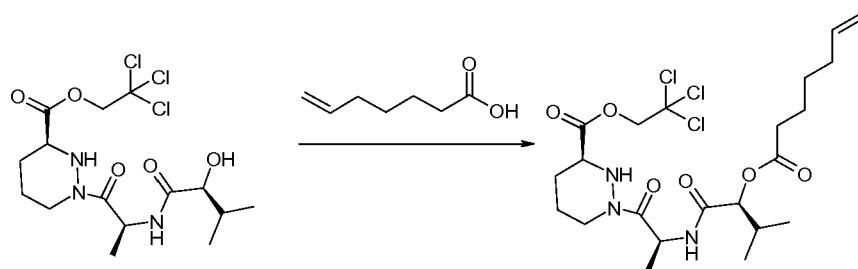
Compound 8a
