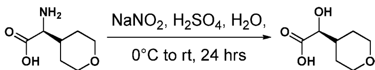
Compound 67a
