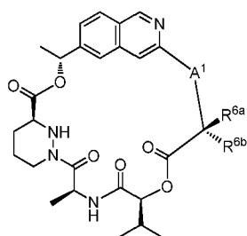
Formula (II-a2)
