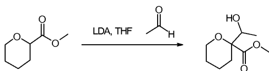
Compound 49a. 2-(1-Hydroxy-ethyl)-tetrahydro-pyran-2-carboxylic acid methyl ester
