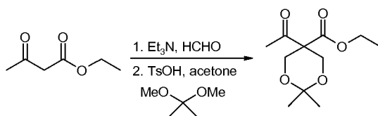
Compound 99a. 5-Acetyl-2,2-dimethyl-[1,3]dioxane-5-carboxylic acid ethyl ester
