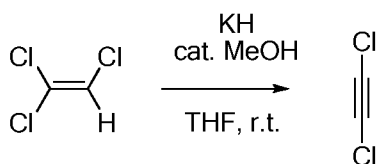
Compound 88a: 1,2-Dichloro-ethyne
