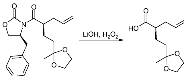
Compound 13a
