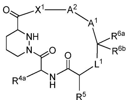
Formula III
