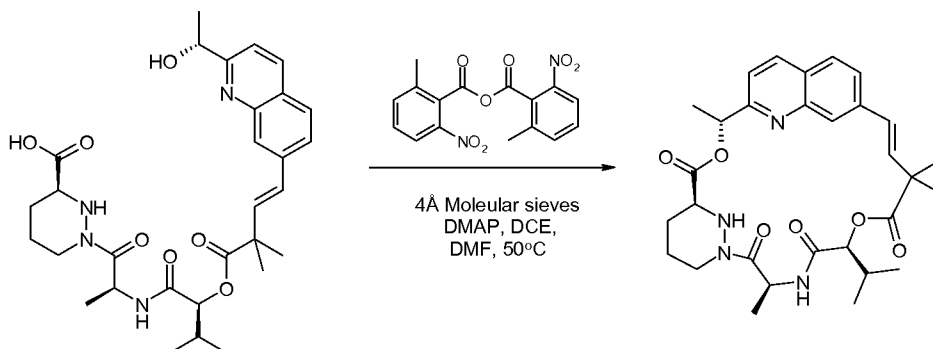
Compound 19
