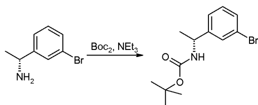
Compound 1h
