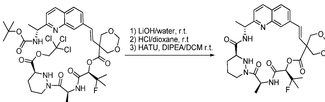
Compound 72
