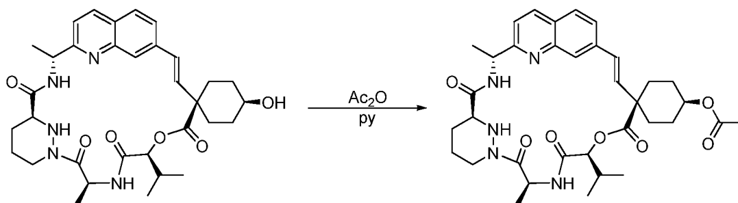
Compound 112
