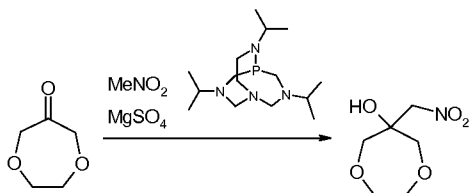
Compound 57a. 6-Nitromethyl-[1,4]dioxepan-6-ol
