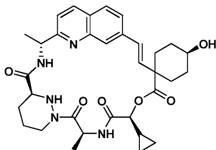
Compound 66a
