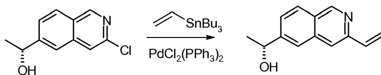
Compound 20b
