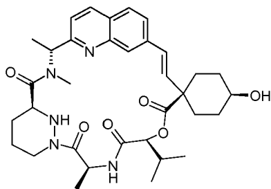
Compound 42a. 4-Oxo-1-vinyl-cyclohexanecarboxylic acid
