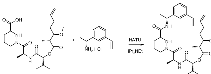
Compound 1k
