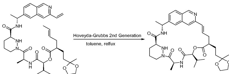
Compound 13
