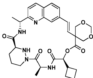
Compound 64a
