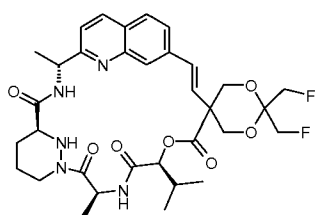
Compound 107a. 2,2-Bis-fluoromethyl-5-vinyl-[1,3]dioxane-5-carboxylic acid ethyl ester
