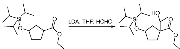
Compound 102b. 1-(1-Hydroxy-ethyl)-3-triisopropylsilanyloxy-cyclopentanecarboxylic acid ethyl ester
