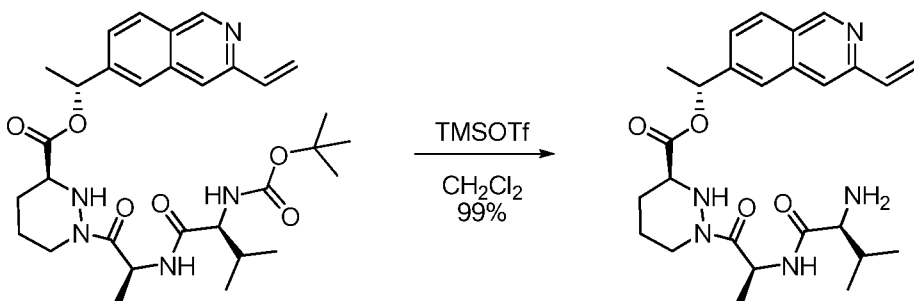
Compound 20f
