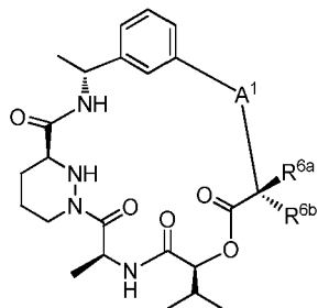
Formula (II-b)
