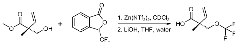
Compound 56a. (R)-2-Methyl-2-trifluoromethoxymethyl-but-3-enoic acid
