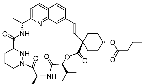
Compound 108
