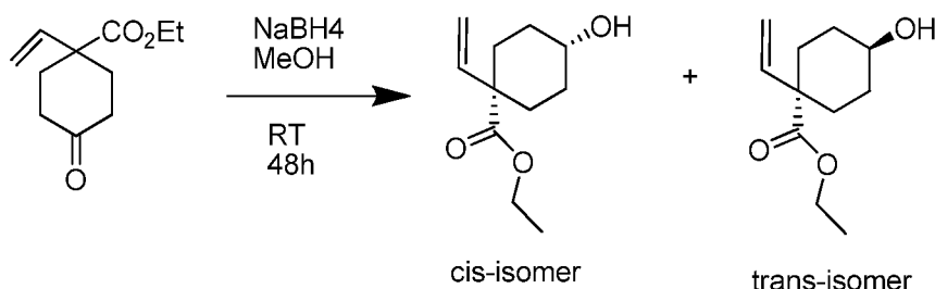
Compound 92a
