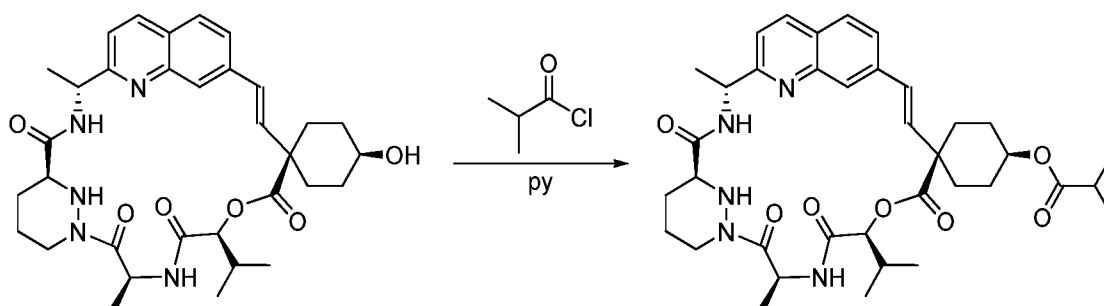
Compound 81
