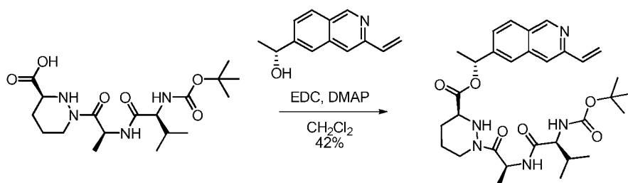
Compound 20e
