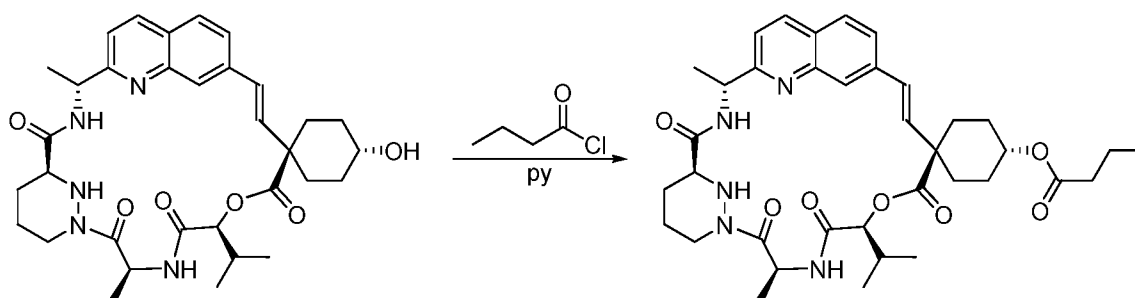
Compound 108
