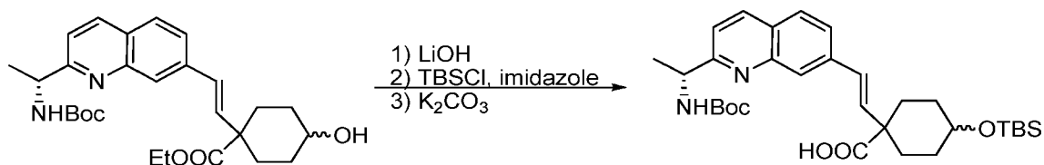
Compound 74c
