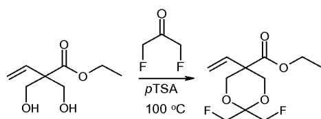
Compound 107a. 2,2-Bis-fluoromethyl-5-vinyl-[1,3]dioxane-5-carboxylic acid ethyl ester
