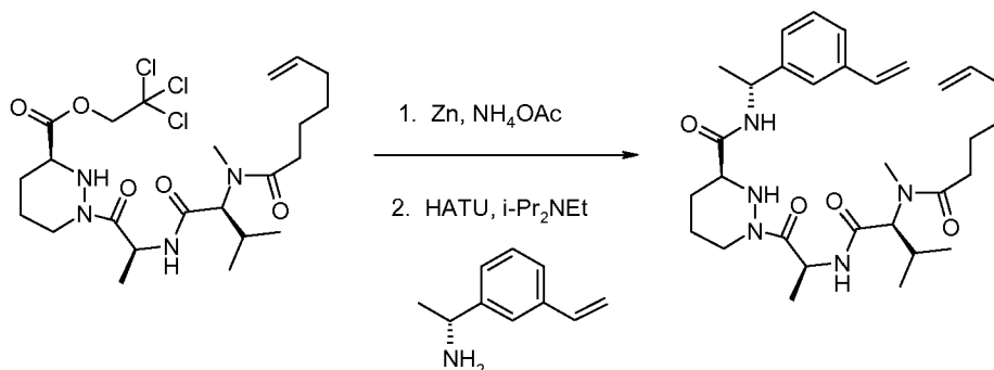
Compound 17c
