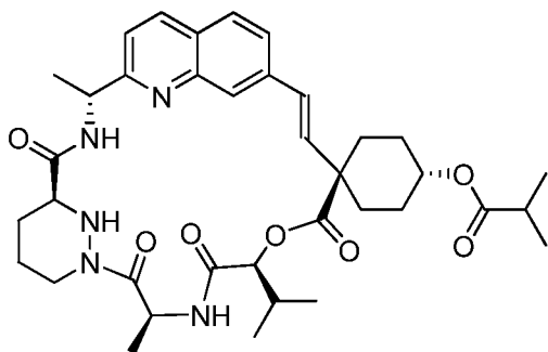
Compound 80
