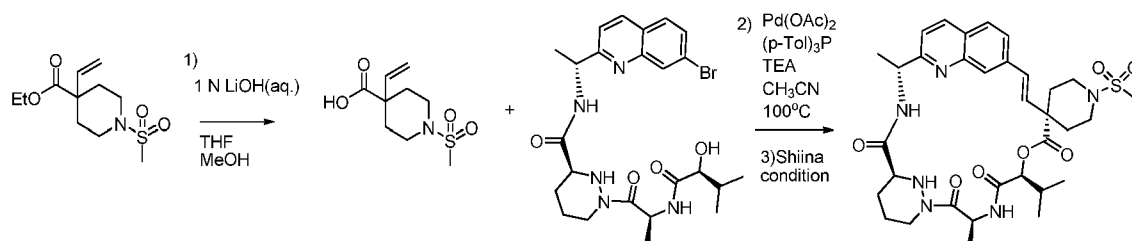
Compound 85
