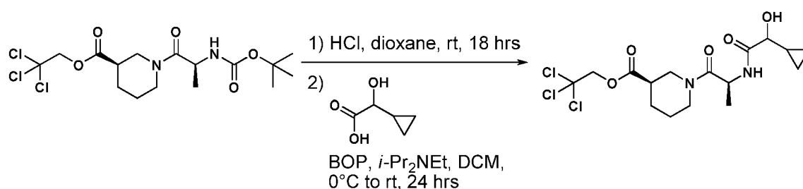
Compound 66a
