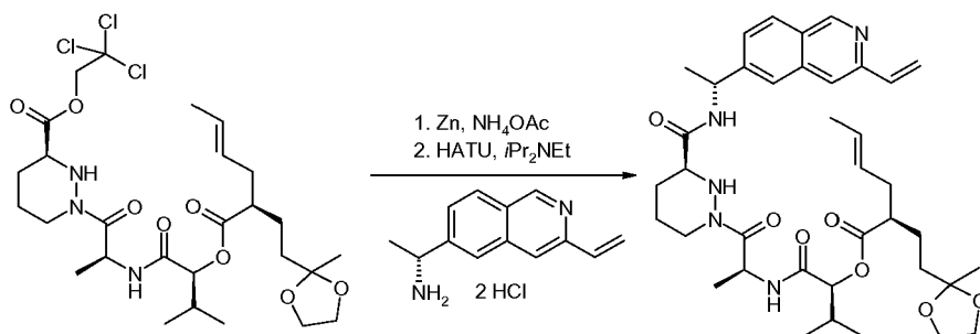
Compound 13c
