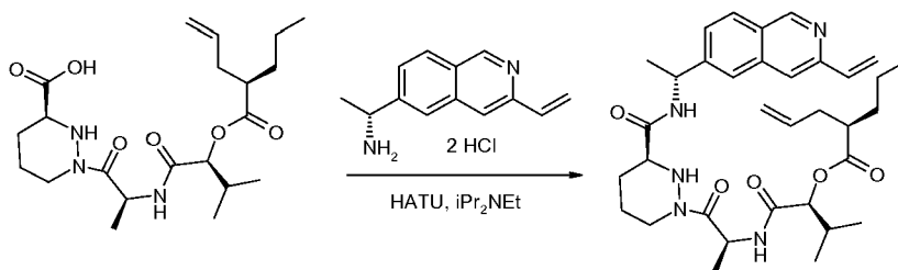
Compound 4f
