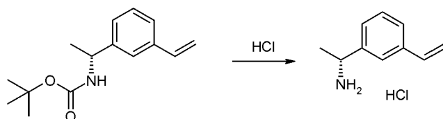
Compound 1j
