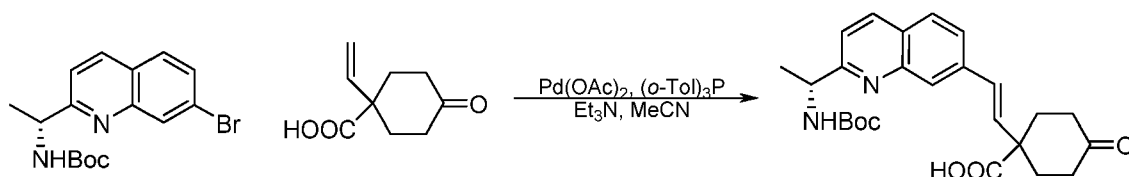
Compound 83a
