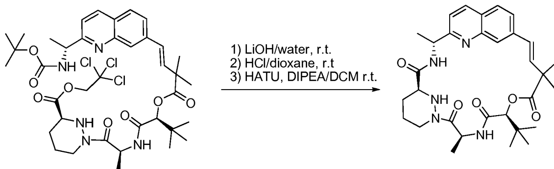
Compound 70
