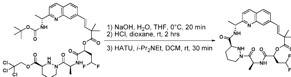
Compound 62
