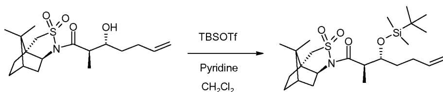
Compound 7a:
