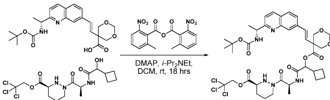
Compound 64b
