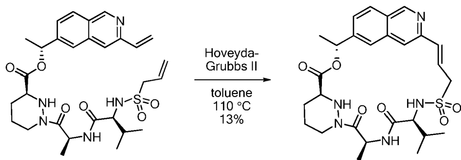
Compound 21
