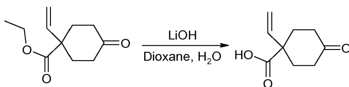
Compound 42a. 4-Oxo-1-vinyl-cyclohexanecarboxylic acid
