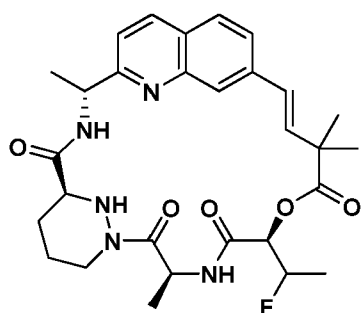
10 Compound 68a
