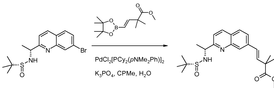
Compound 18d
