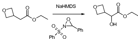
Compound 95a. Hydroxy-oxetan-3-yl-acetic acid ethyl ester
