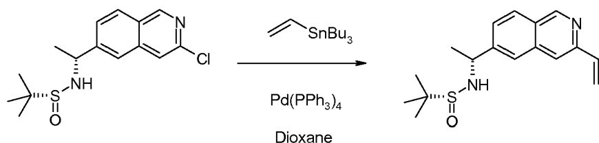
Compound 2i
