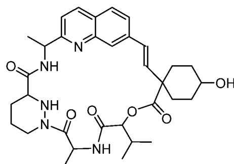
Compounds 76 and 77
