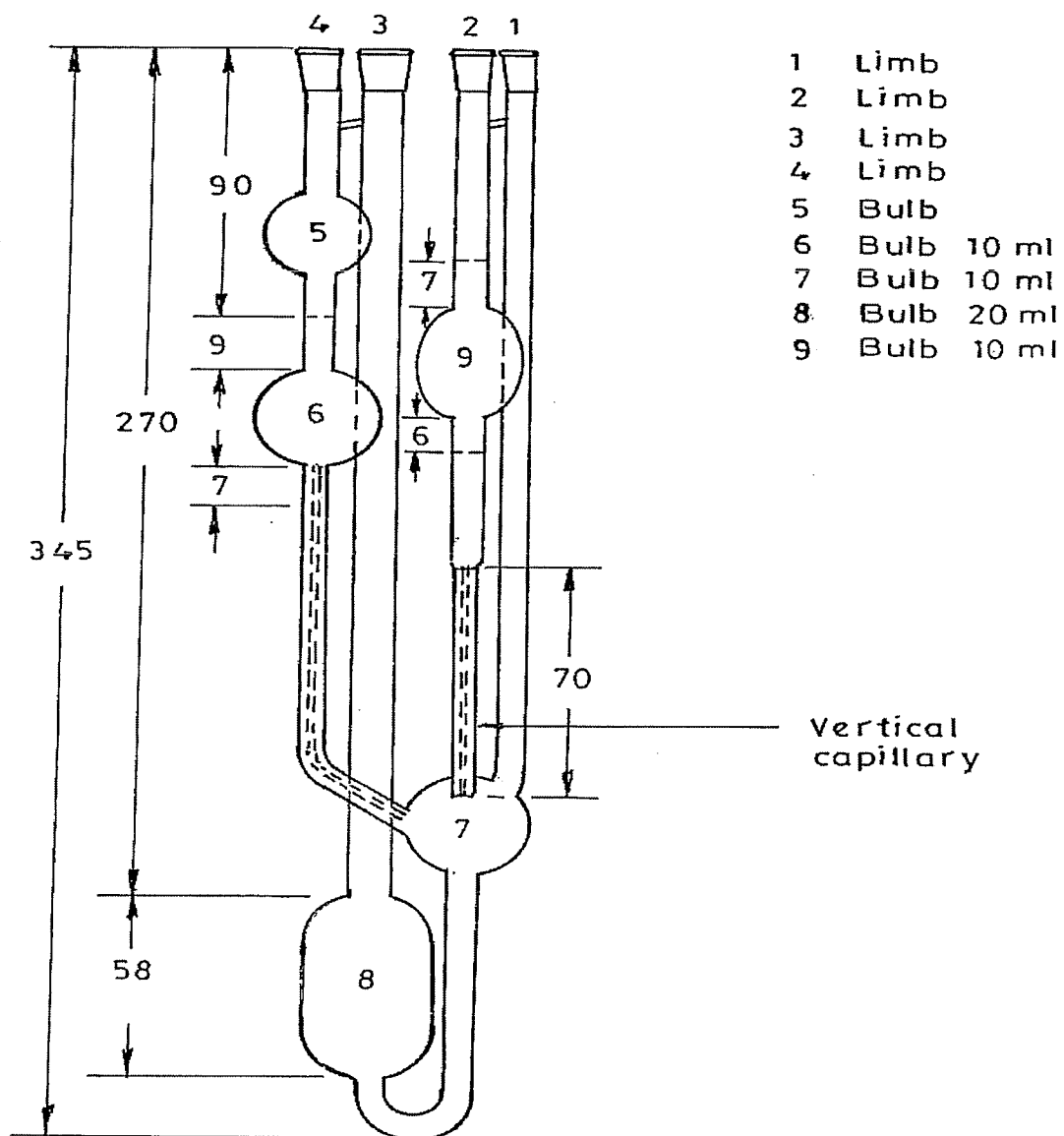
SURVISMETER -TYPE 1
