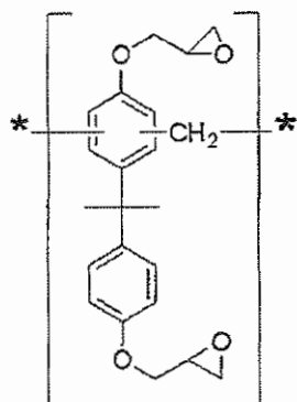
JER-157S65
