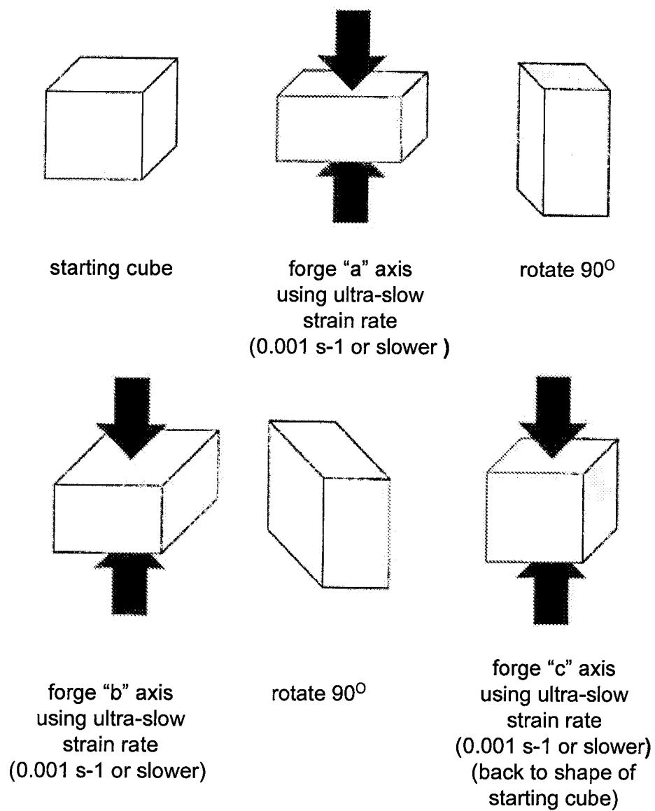
FIG. 4 PRIOR ART
