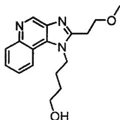
4-(2-(2-Methoxyethyl)-1H-imidazo[4,5- c ]quinolin-1-yl)butan-1-ol
