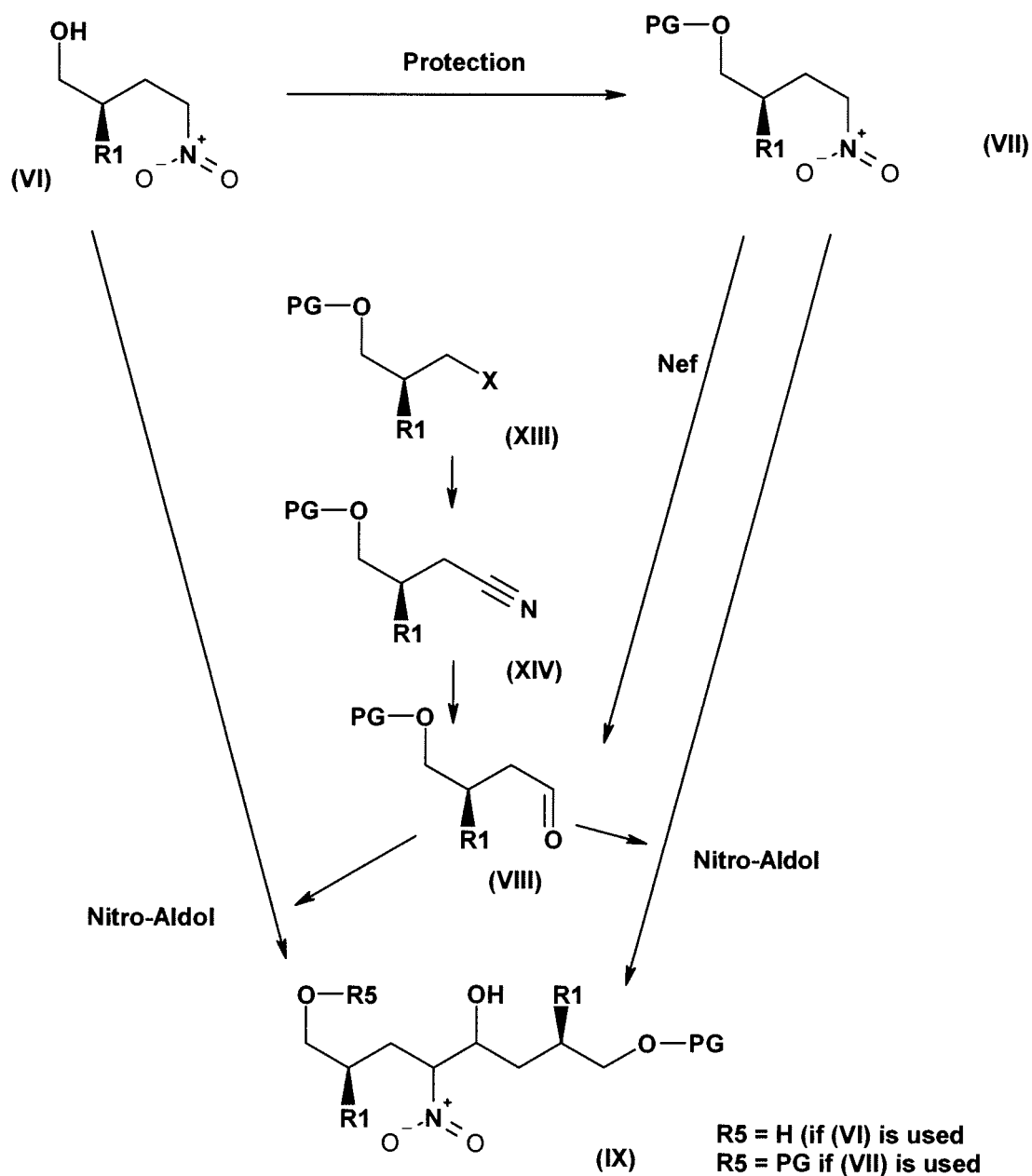
Scheme 2: Overview of routes to nitro-aldol reaction
