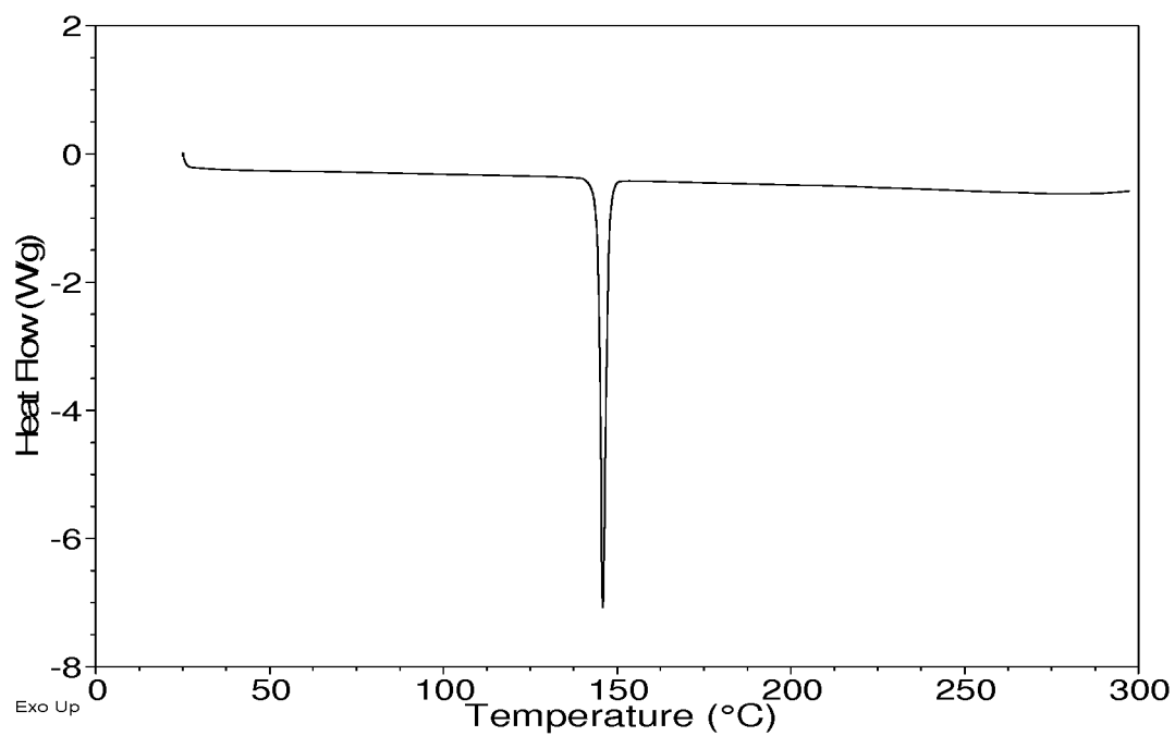
Figure 4: DSC Thermogram of Form B of 7-Fluoro-1-isopropyl-3-methyl-8-[6-[3-(1-piperidyl)propoxy]-3-pyridyl]imidazo[4,5-c]quinolin-2-one
