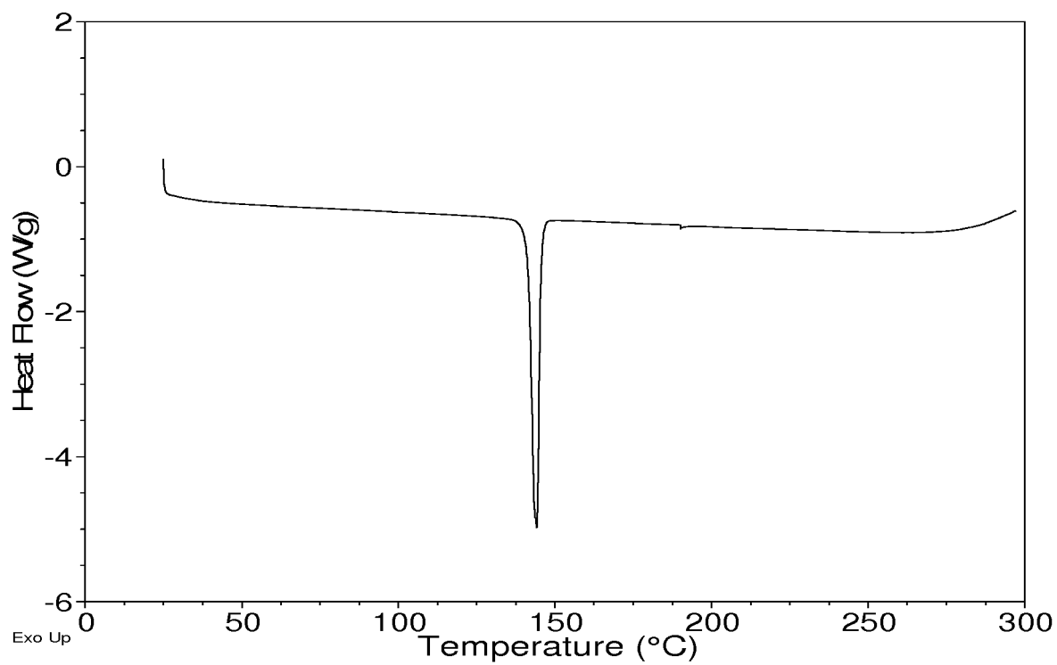
5 Figure 2: DSC Thermogram of Form A of 7-Fluoro-1-isopropyl-3-methyl-8-[6-[3-(1-piperidyl)propoxy]-3-pyridyl]imidazo[4,5-c]quinolin-2-one
