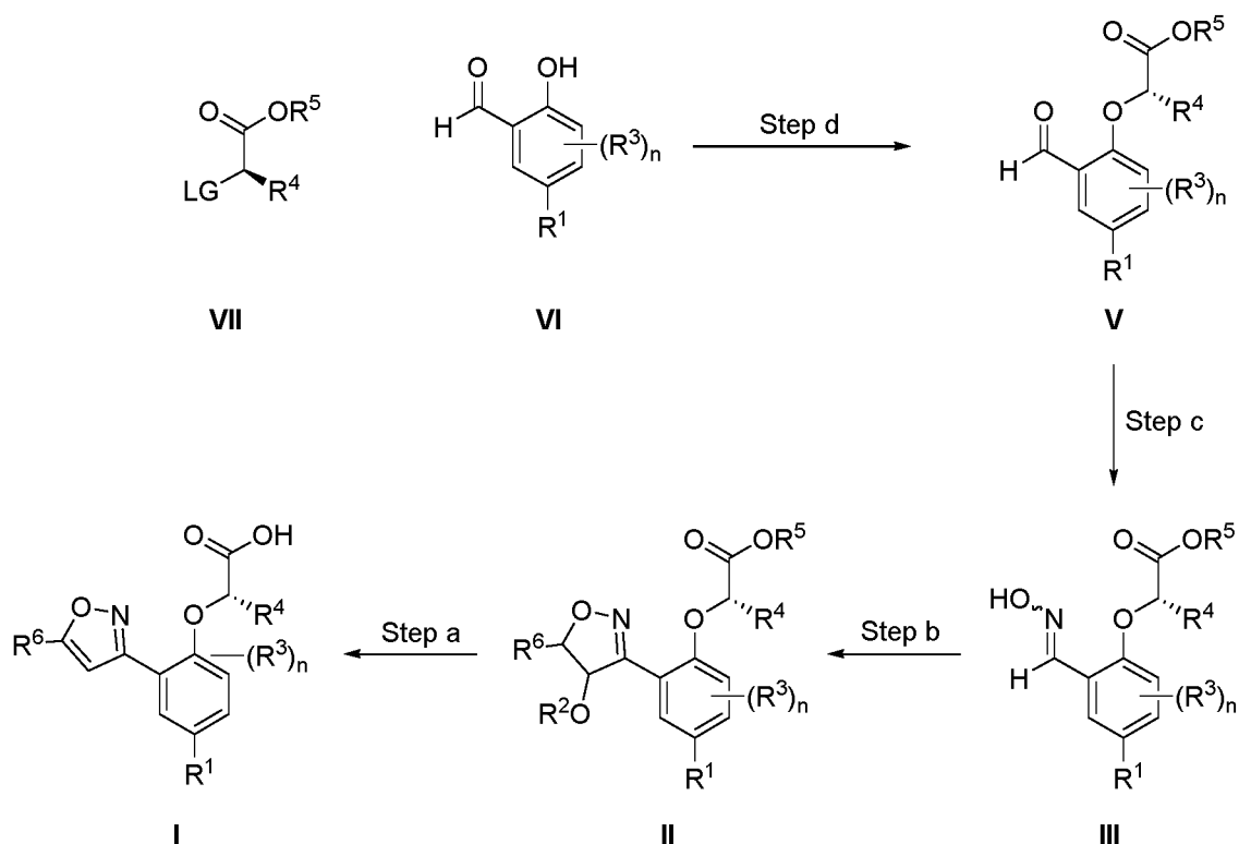
15 Scheme 1: Synthesis of compounds of Formula I
