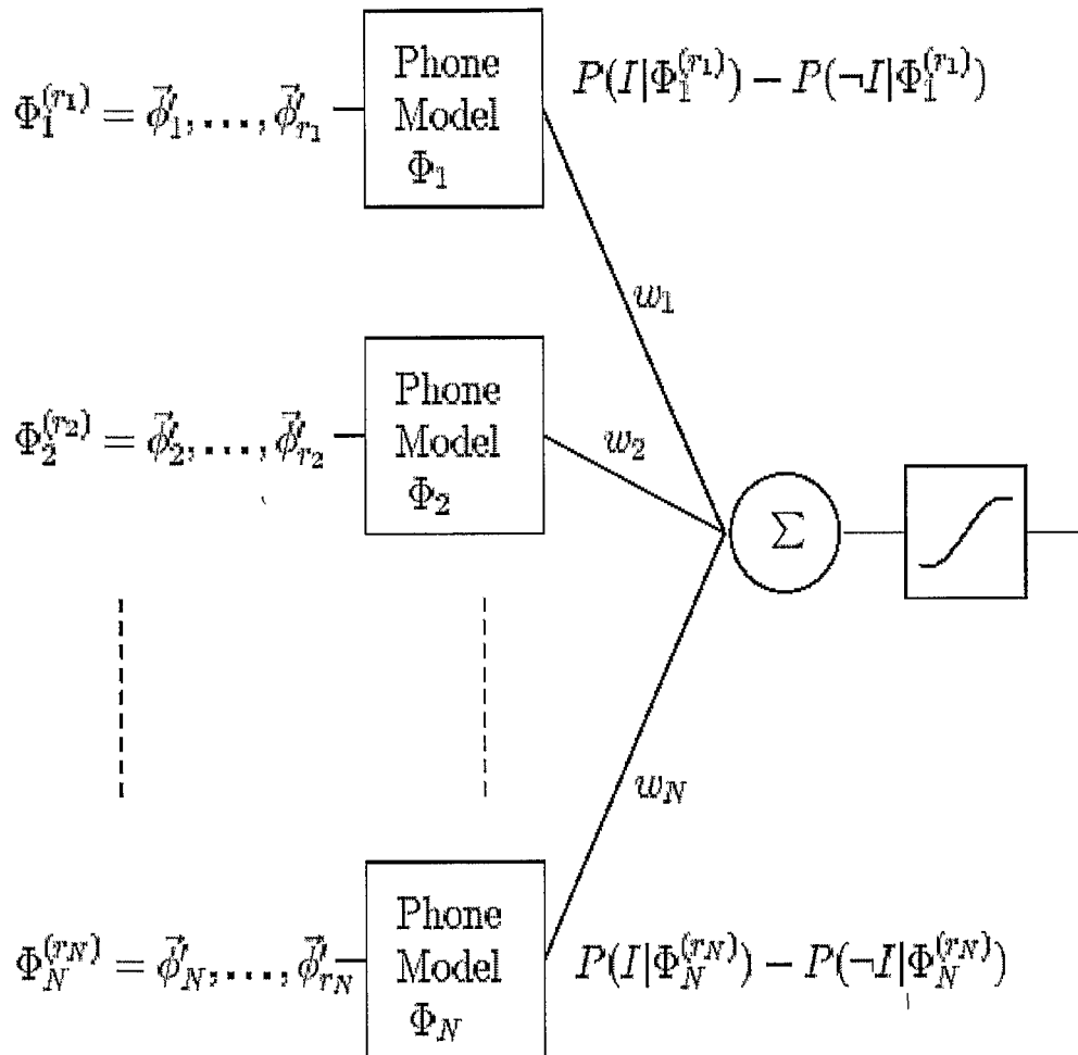
Figure: 2 A super classifier
