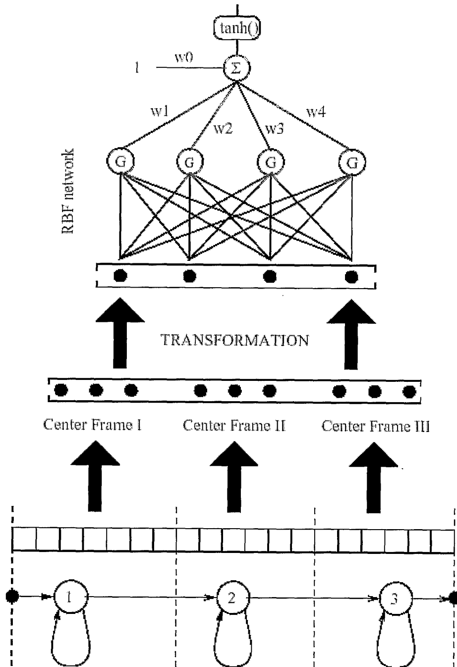
Figur 7: RBF network
