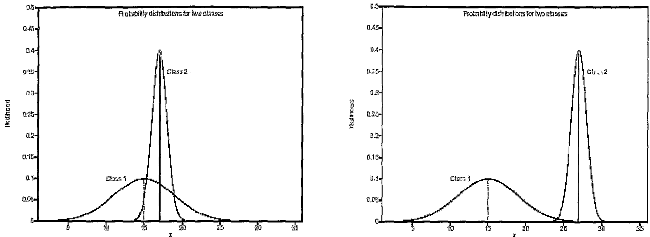
Figure 2 Two classes were the Bayes classifier uses quadratic decision surfaces.
