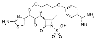
Epimer B
