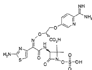
Epimer B
