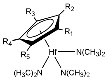
[Chemical Formula 5]
