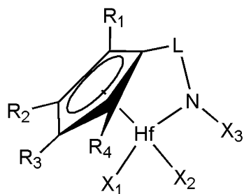
[Chemical Formula 6]
