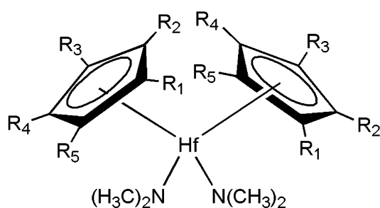
[Chemical Formula 6]
