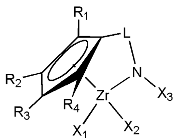
[Chemical Formula 4]
