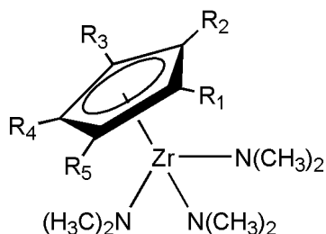
[Chemical Formula 2]
